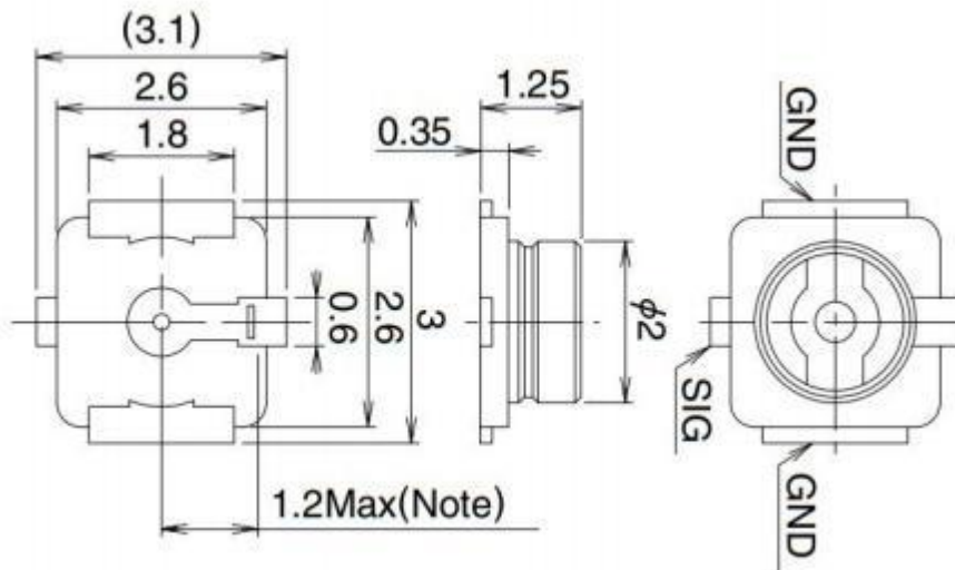
Figure 7: u.FL-R-SMT-1(80) Dimensions
