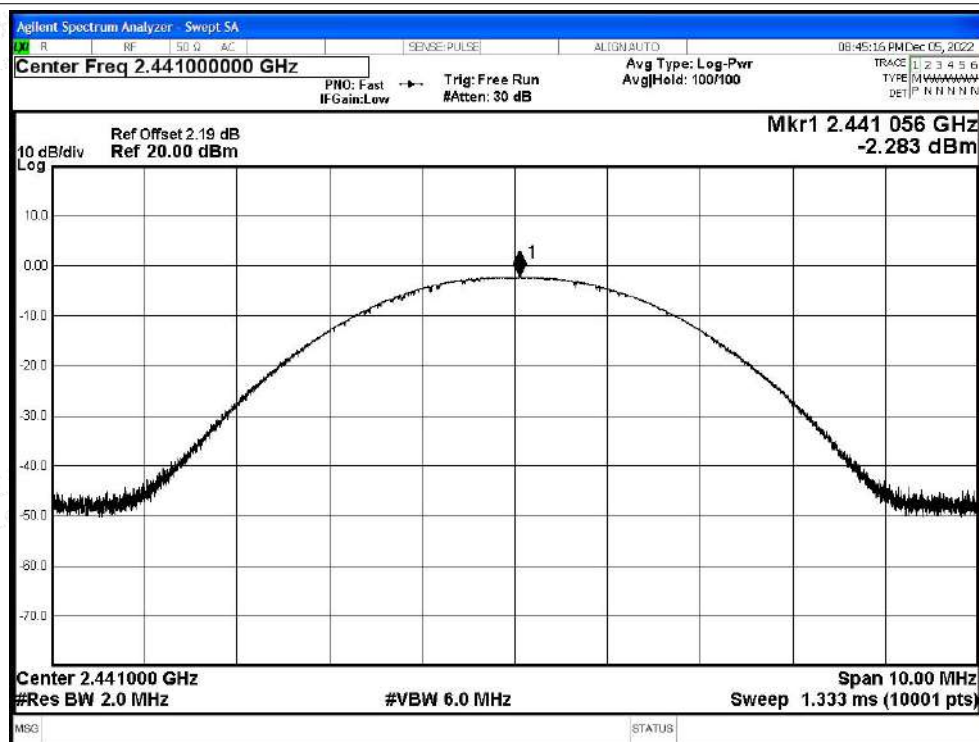
Power NVNT 3-DH5 2441MHz Ant5
