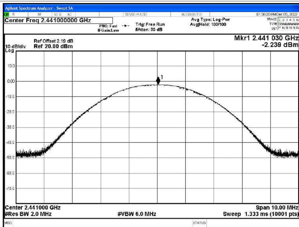
Power NVNT 3-DH5 2441MHz Ant4
