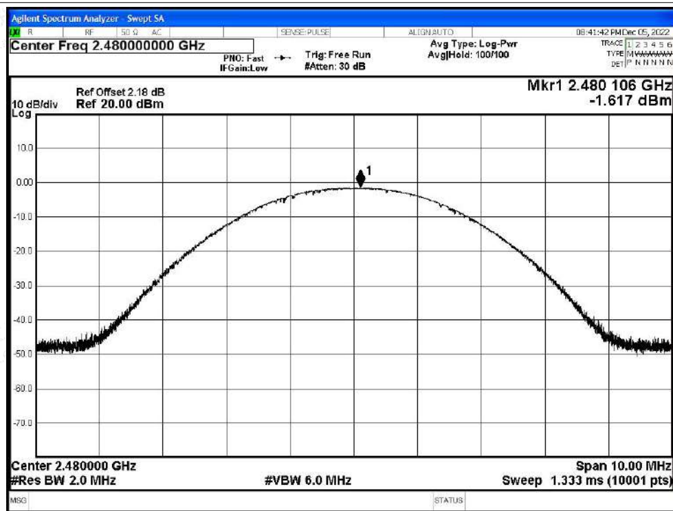
Power NVNT 2-DH5 2480MHz Ant5
