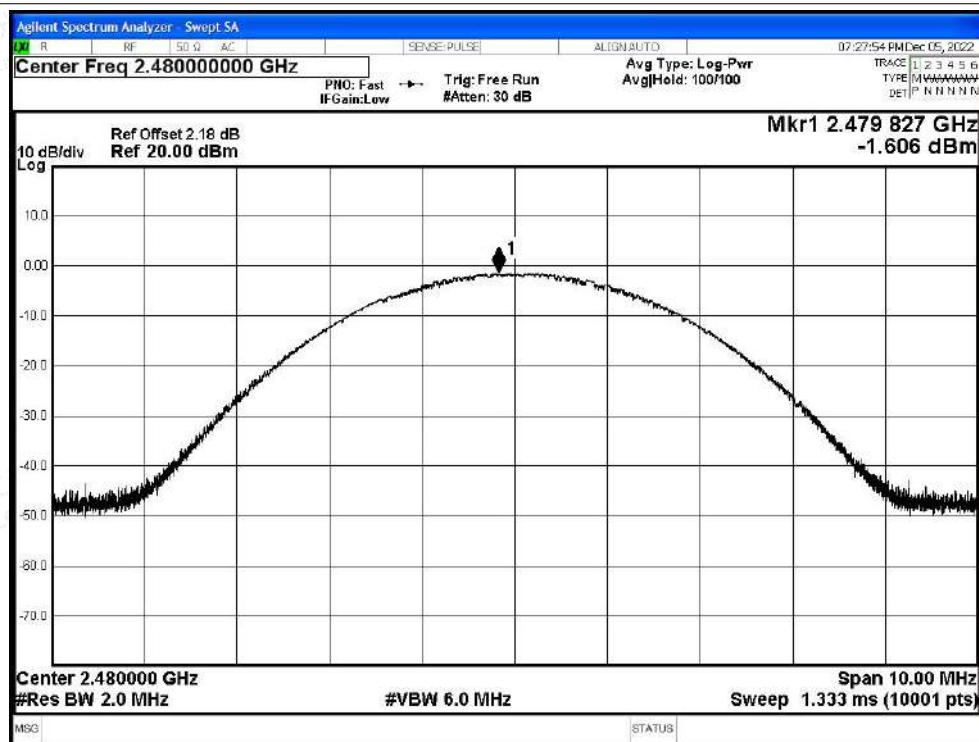
Power NVNT 2-DH5 2480MHz Ant4
