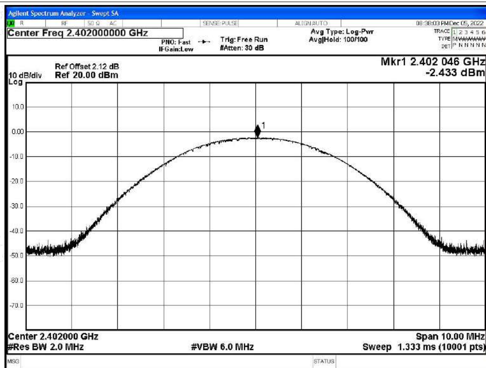
Power NVNT 2-DH5 2402MHz Ant5
