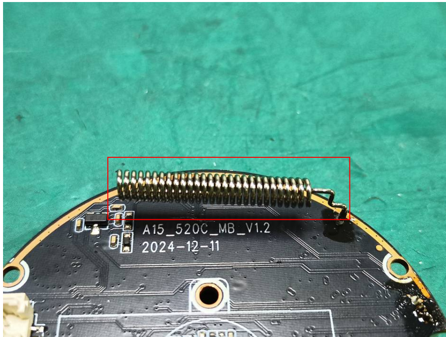
433.92MHz TX ANT
