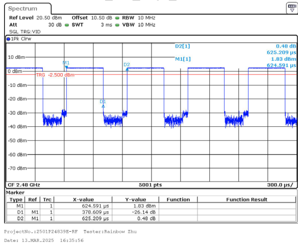
BLE_1M_High_Channel
