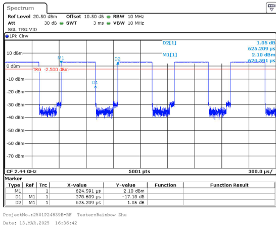
BLE_1M_Middle_Channel
