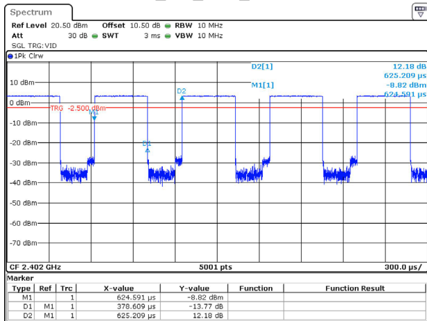
BLE_1M_Low_Channel
