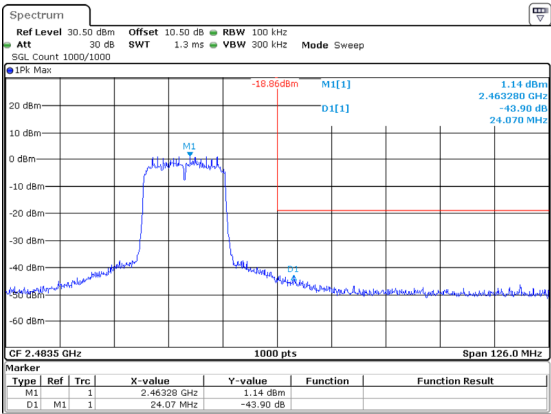
802.11ax20_2462MHz_RU_Full
