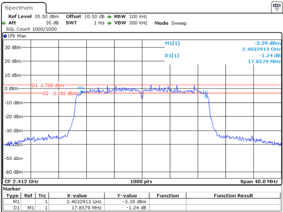
802.11ax20_2412MHz_RU_Full
