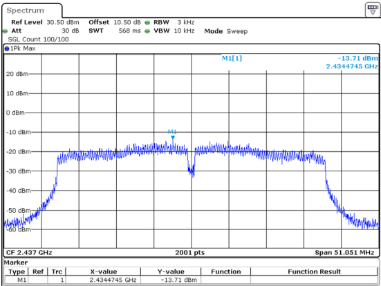
802.11n40_2437MHz
