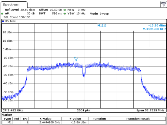
802.11n40_2452MHz
