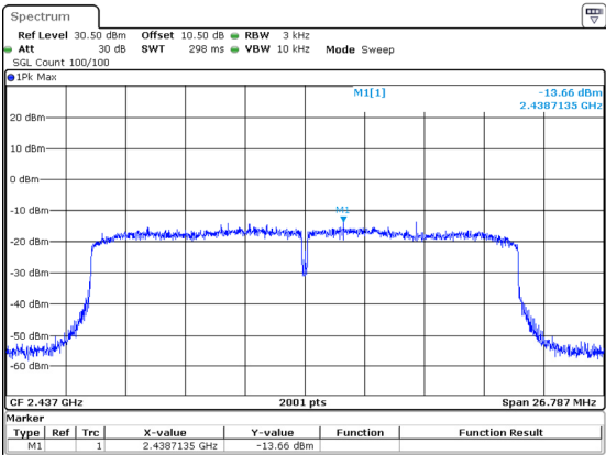
802.11ax20_2437MHz_RU_Full
