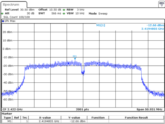
802.11n40_2422MHz
