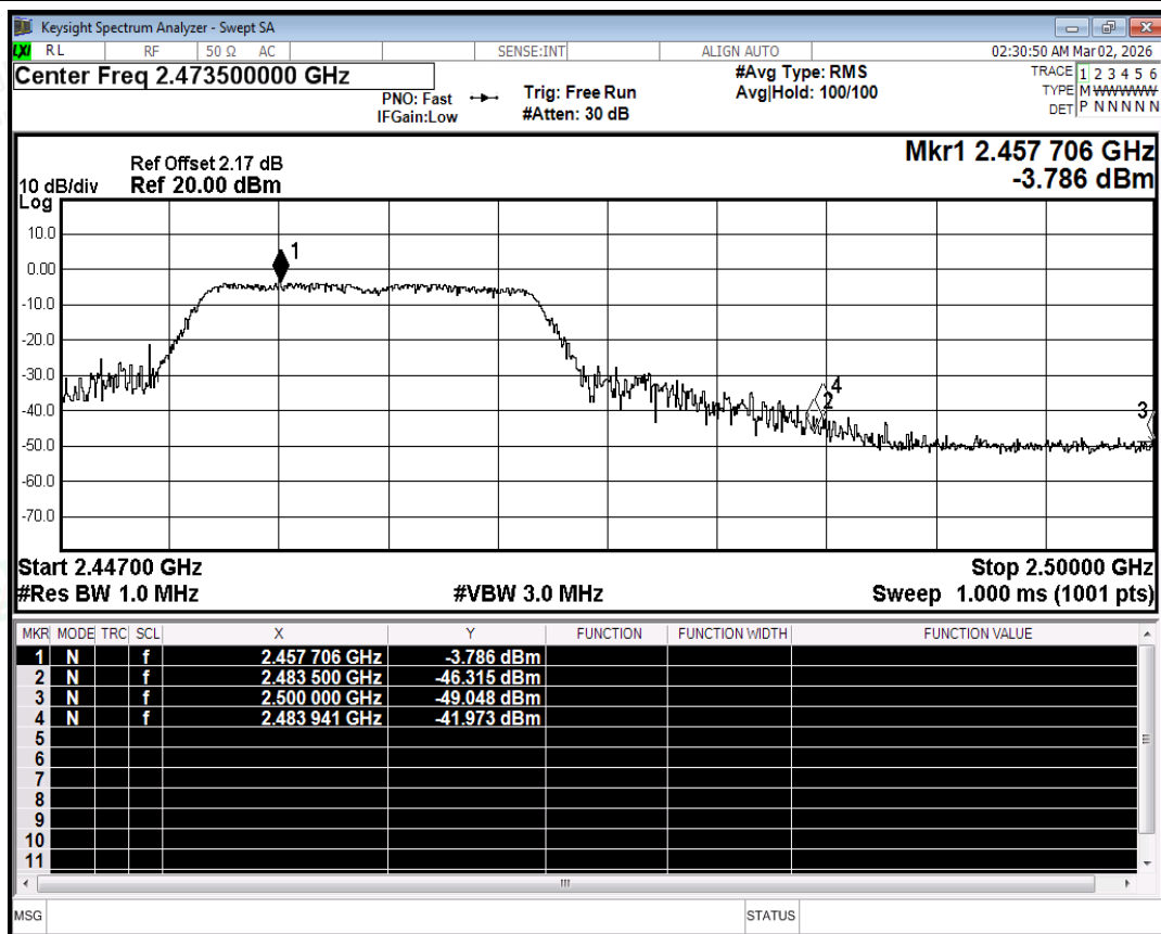
Restrict Band NVNT g 2462MHz Ant1 Peak
