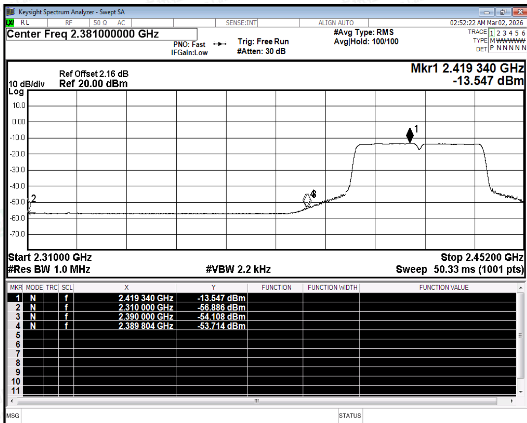
Restrict Band NVNT ax40 2422MHz Ant1 Average
