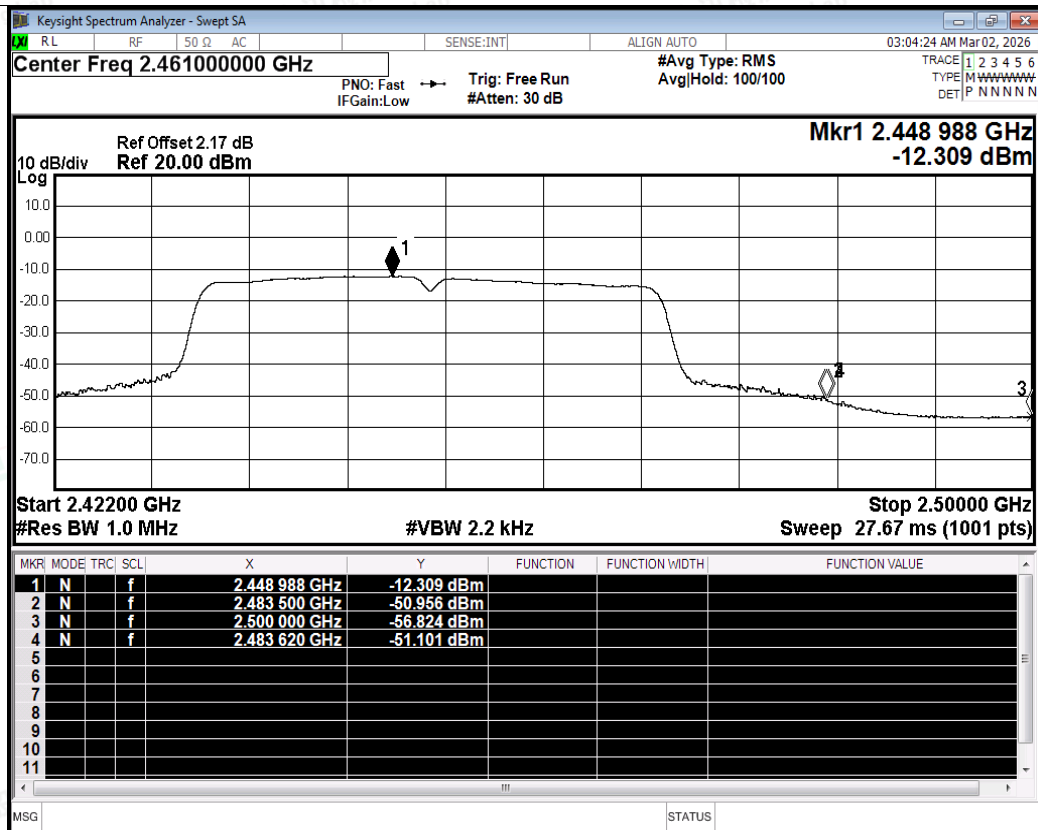
Restrict Band NVNT ax40 2452MHz Ant1 Average
