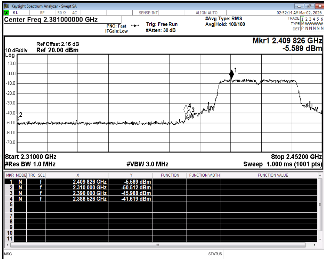
Restrict Band NVNT ax40 2422MHz Ant1 Peak
