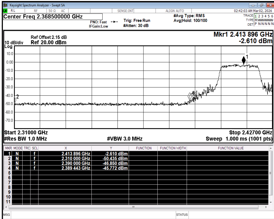
Restrict Band NVNT ax20 2412MHz Ant1 Peak
