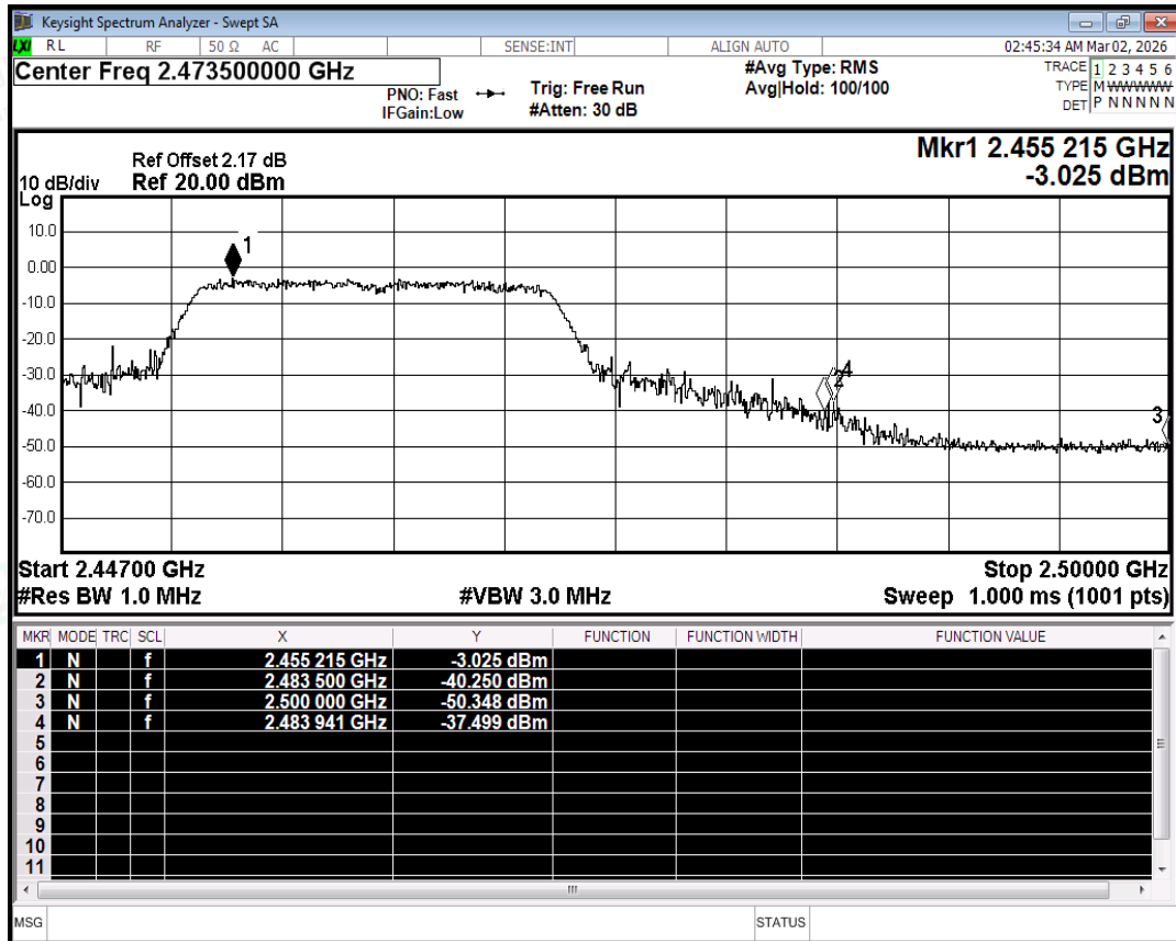
Restrict Band NVNT ax20 2462MHz Ant1 Peak
