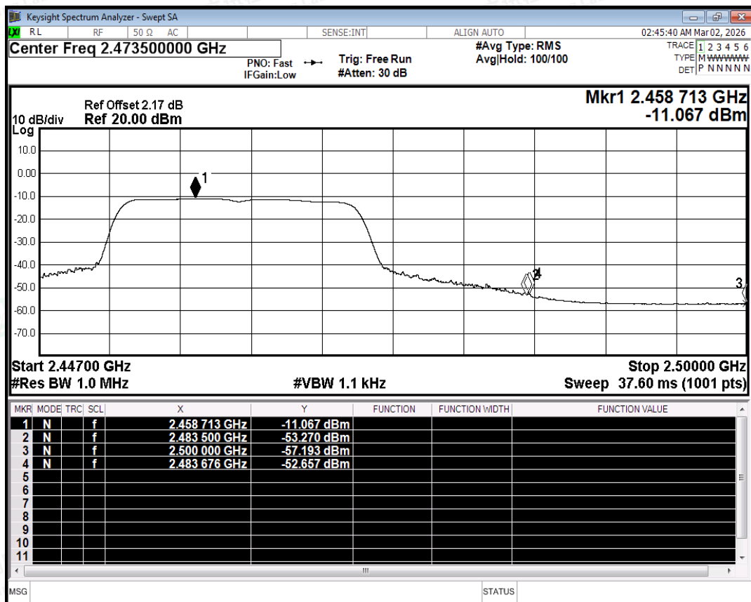
Restrict Band NVNT ax20 2462MHz Ant1 Average
