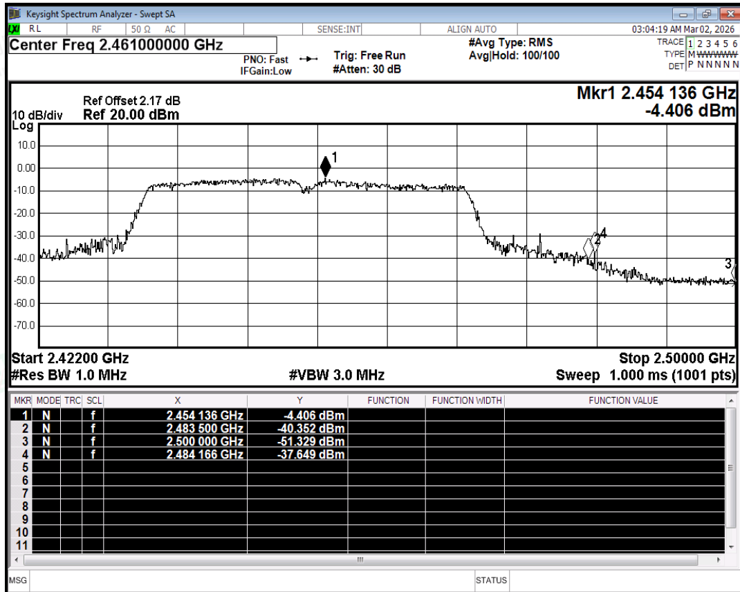
Restrict Band NVNT ax40 2452MHz Ant1 Peak
