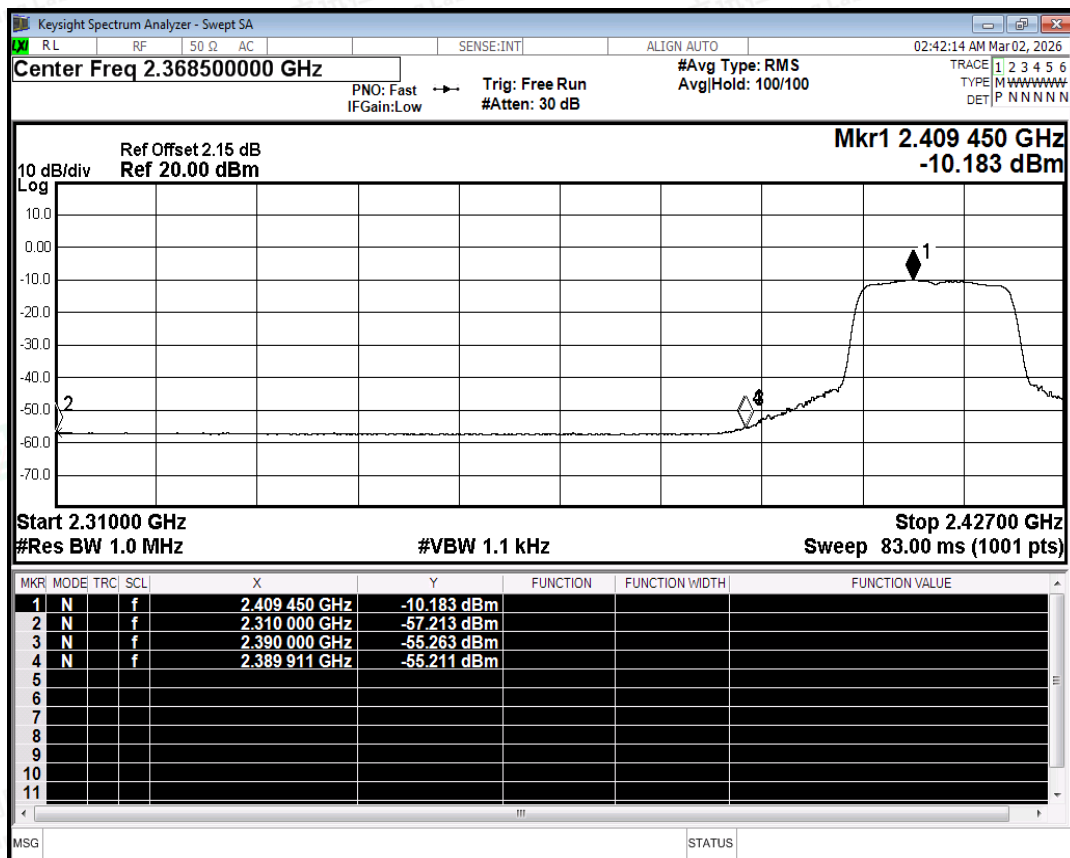
Restrict Band NVNT ax20 2412MHz Ant1 Average
