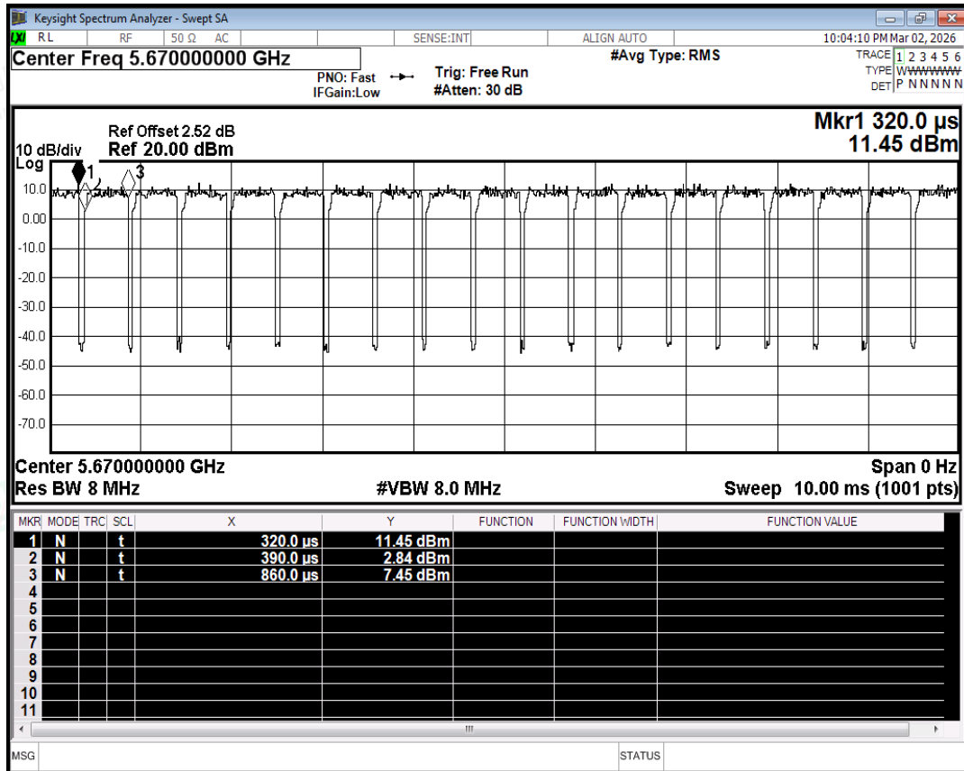
Duty Cycle NVNT ax40 5670MHz Ant1
