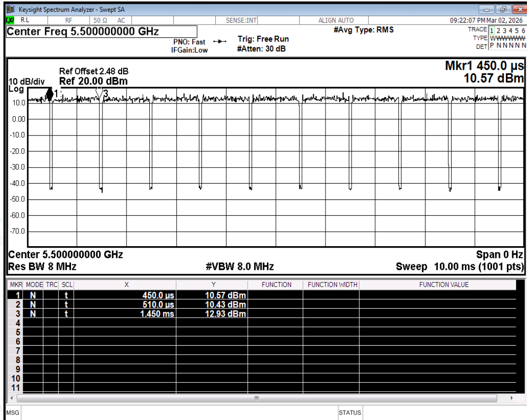
Duty Cycle NVNT ax20 5500MHz Ant1
