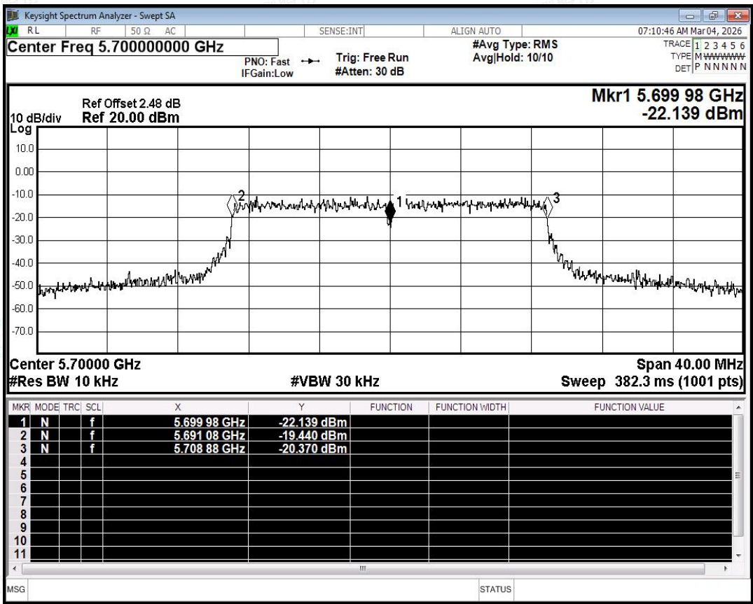
Freq. Stability NVNT ac20 5700MHz Ant1
