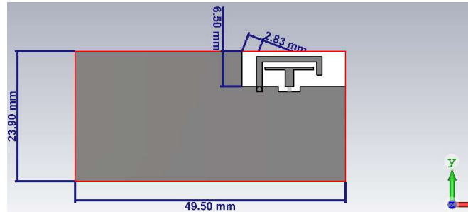
Figure 1: Antenna design
