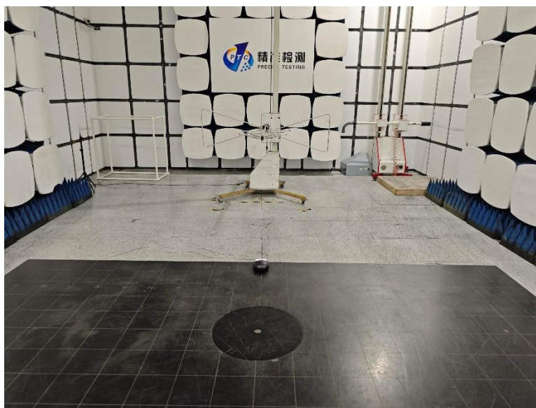
Radiated Emissions Test(Below 1G)
