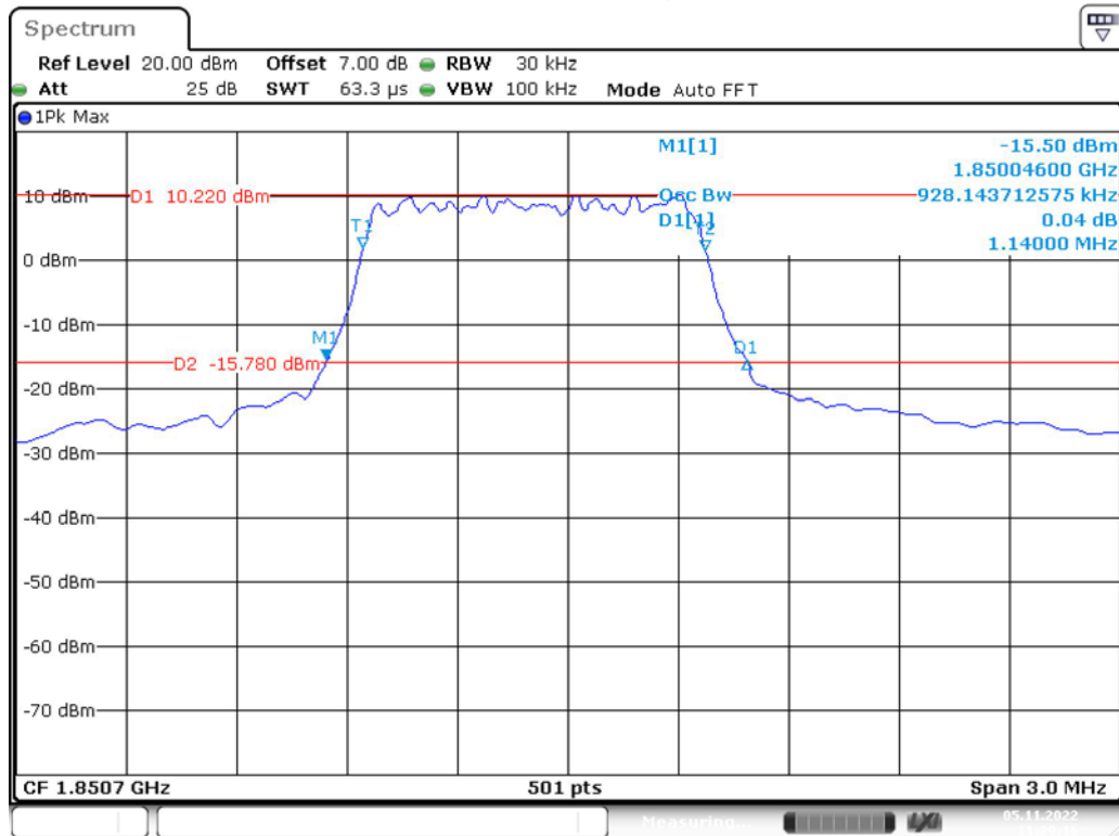
Band 2_1.4 MHz_Low_16QAM_RB5#0
