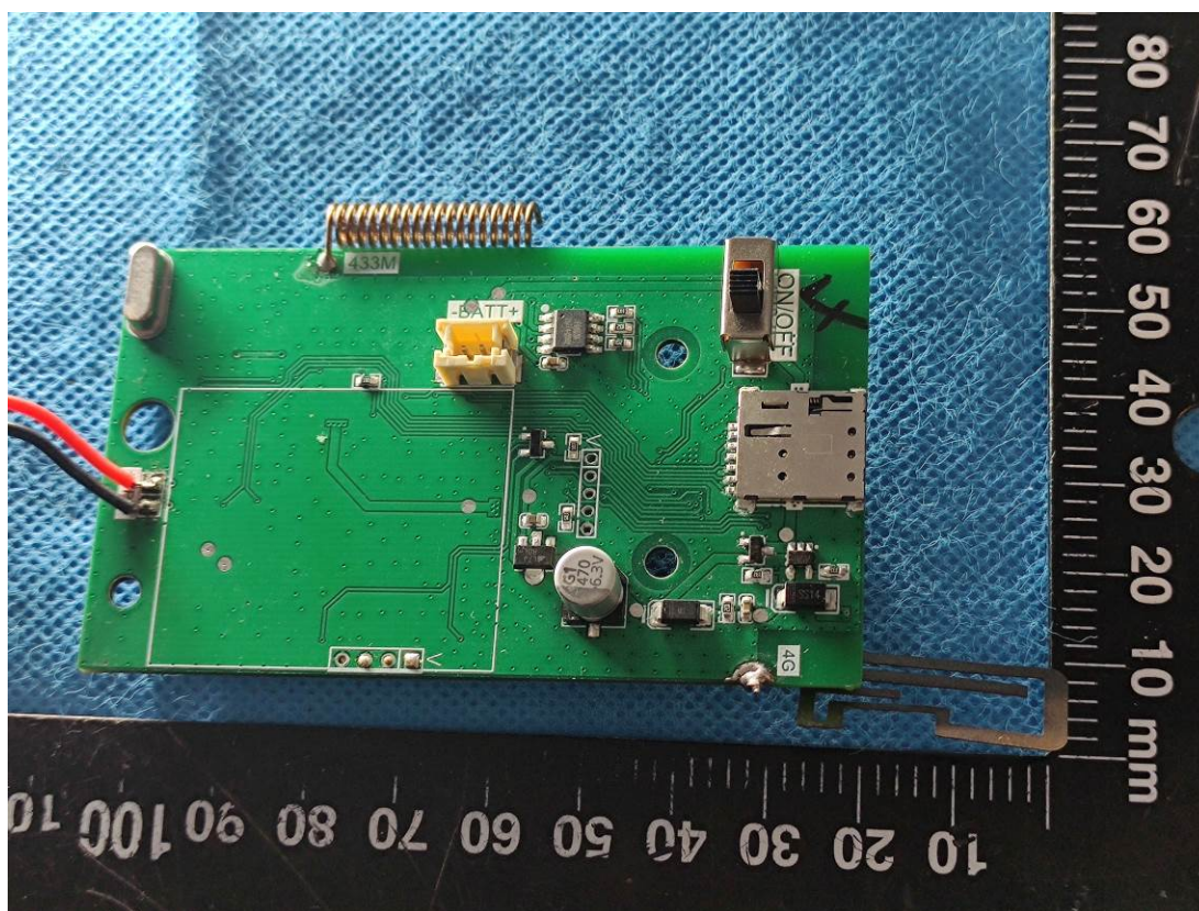
433M Receiver Antenna
