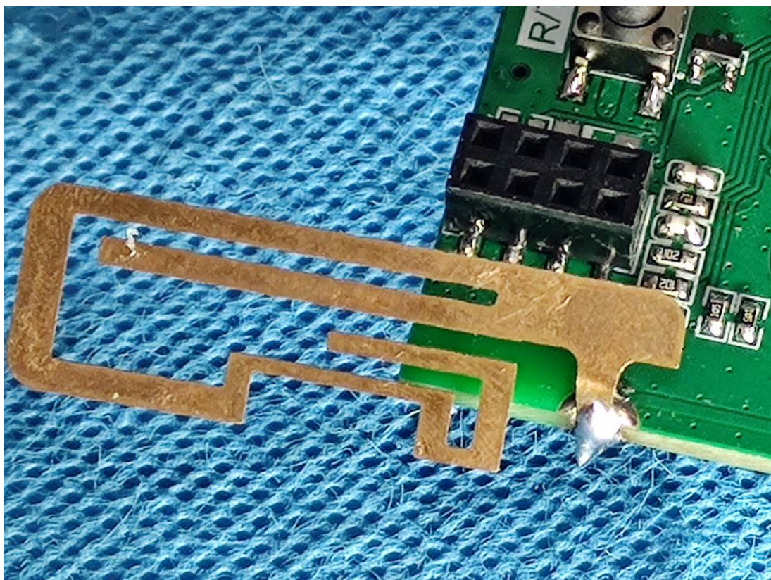
NB-IoT Antenna
