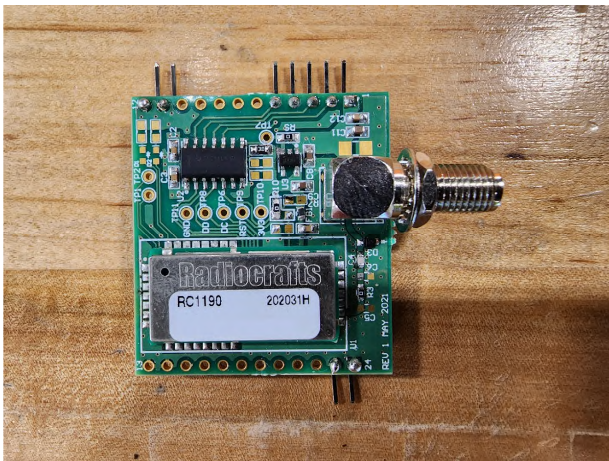
Figure 1 – Front without Antenna
