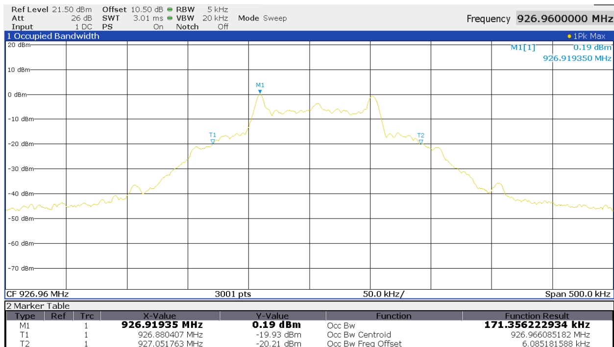
Figure 3 – 99% Bandwidth - High Channel
