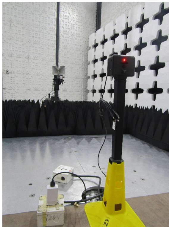
Emission (Above 1000MHz)
