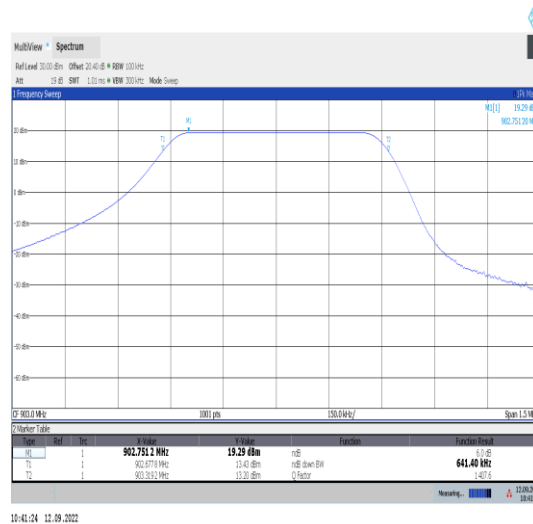
Bottom Channel_903 MHz
