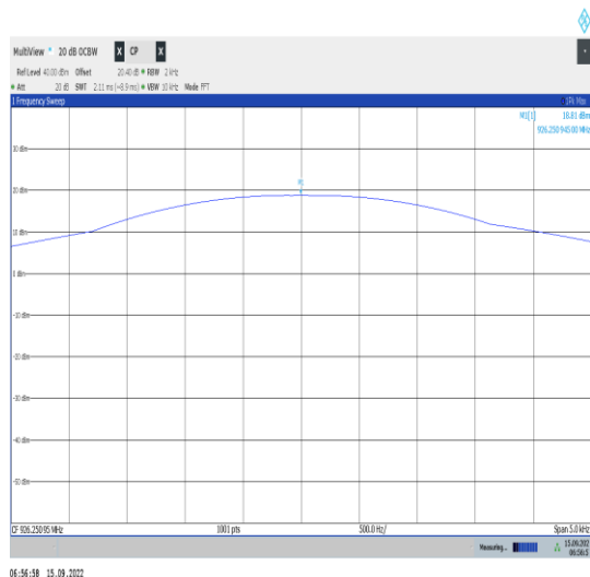
Hopping Channel - 926.25095 MHz
