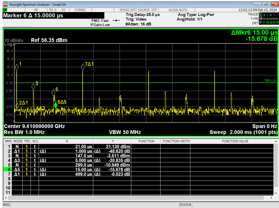
Figure 47 – Pulse length plot, shows shortest pulse length observed
