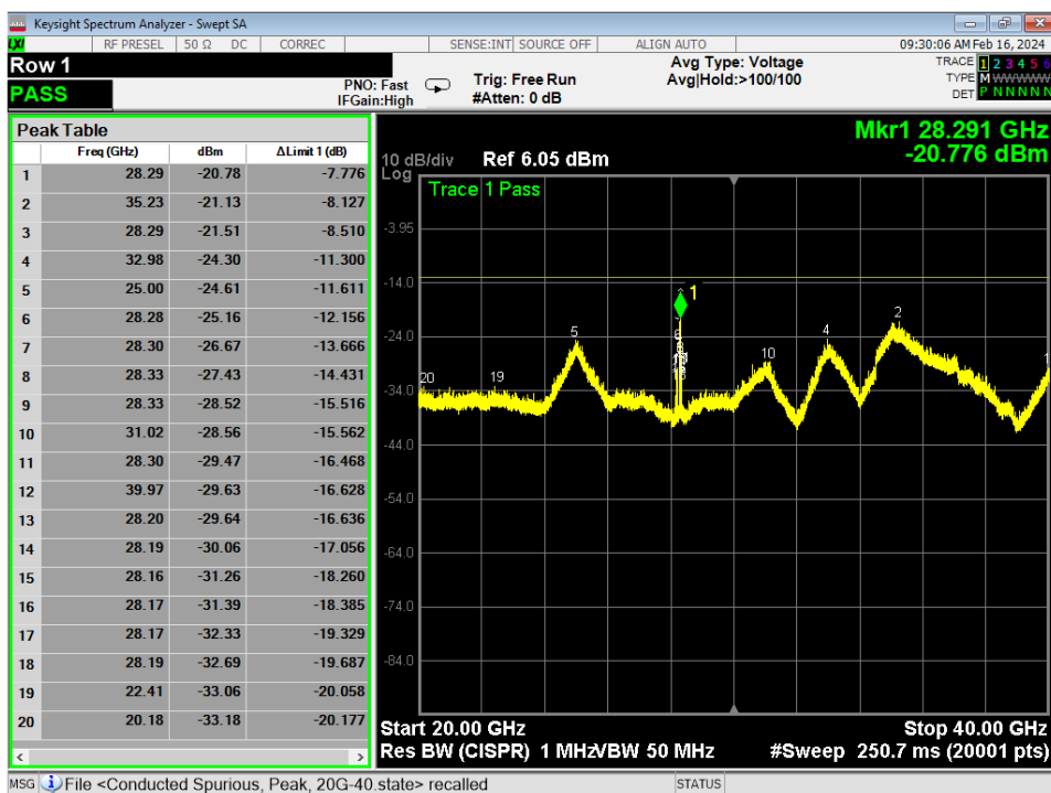
Figure 24 - Conducted Unwanted Emissions Plot, 20GHz-40GHz, Mode C *Limit is -13dB – Pass
