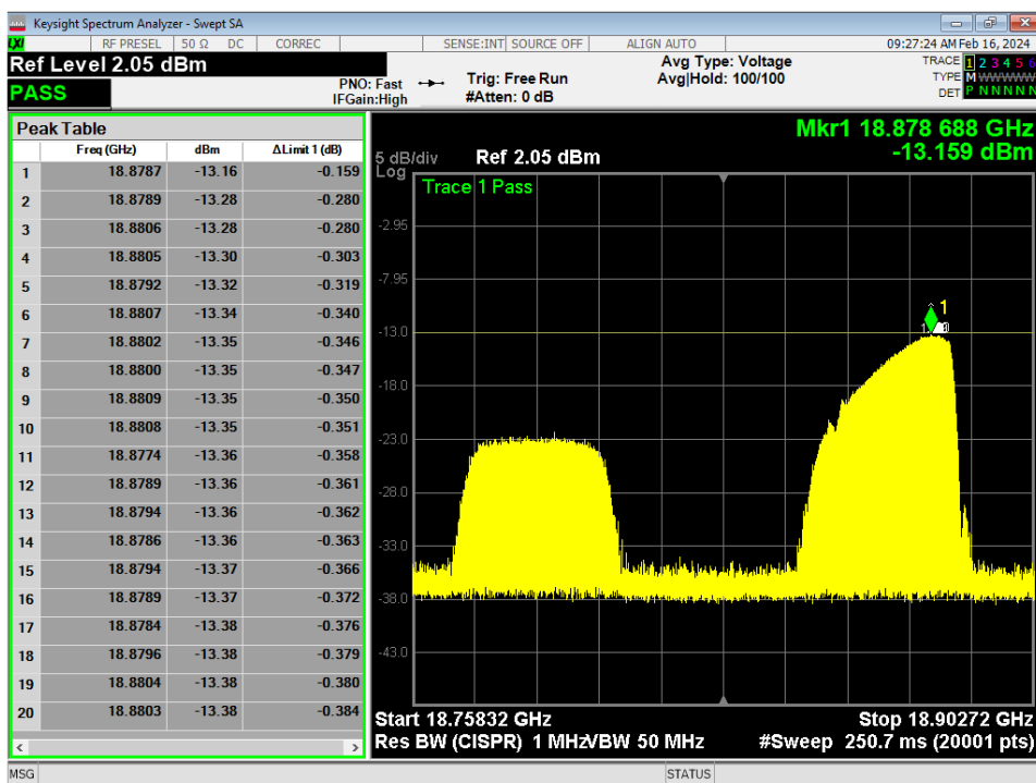
Figure 23 - Conducted Unwanted Emissions Plot, 18.75832GHz-18.90272GHz, Mode C *Limit is -13dBm – Pass
