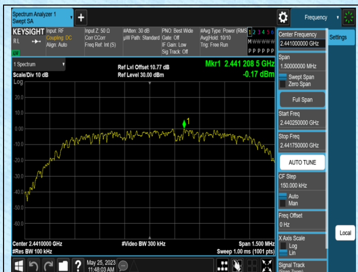
2DH5-Ant1-2441-0~Reference
