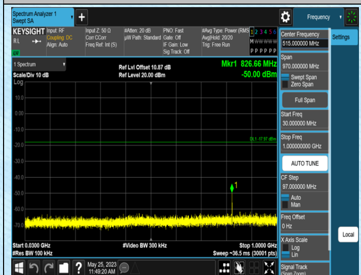
2DH5-Ant1-2480-30~1000
