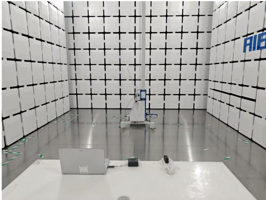
Radiated Spurious Emission Test View 1
