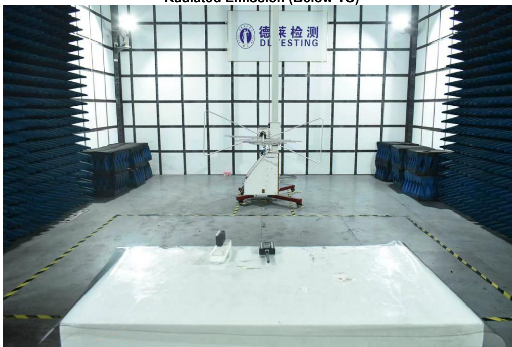
Radiated Emission (Below 1G)
