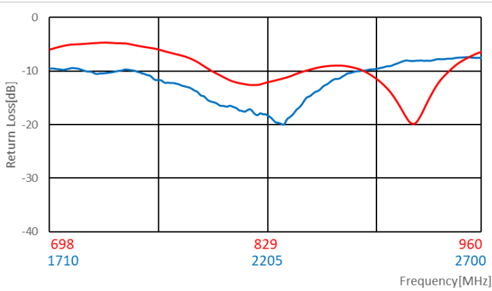
Return Loss
