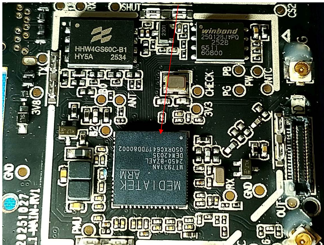
BLE&5.8G Wifi Chip
