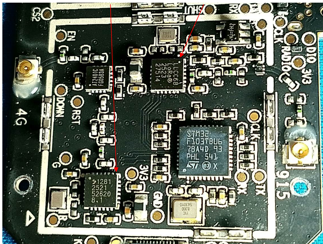
900M Lora Chip
