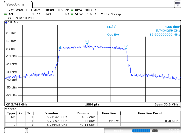
802.11ax20_5745MHz_RU_Full
