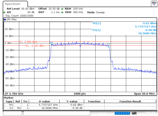
802.11ax20_5785MHz_RU_Full
