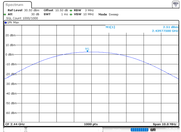
BLE_1M_Middle_Channel
