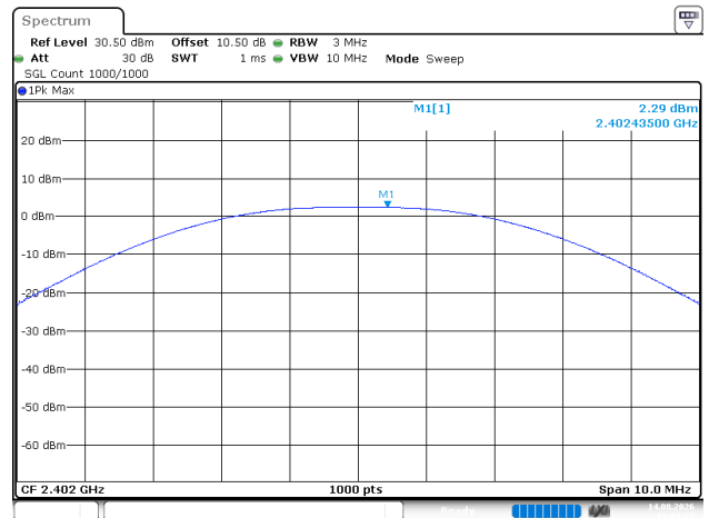
BLE_2M_Low_Channel
