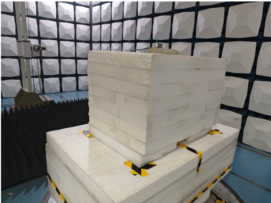
Radiated Emission Above 1GHz View 18-26.5G
