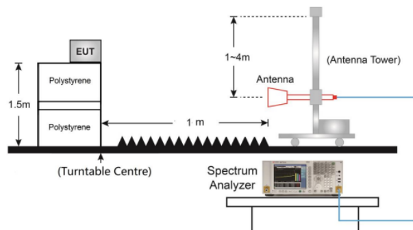
1GHz ~ 40GHz Test Setup:
