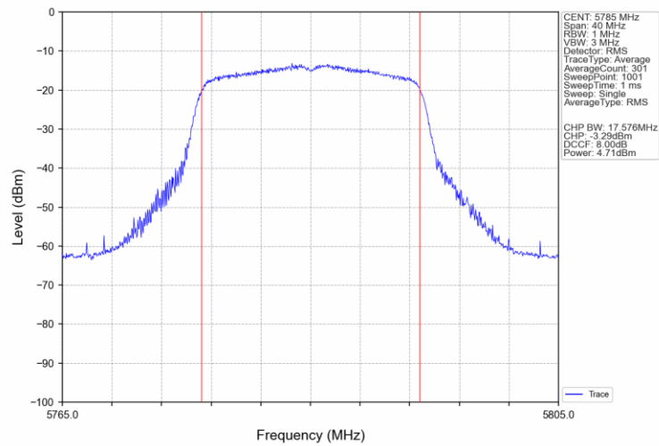
802.11n(HT20)_MCH_5785MHz_Ant2_NTNV
