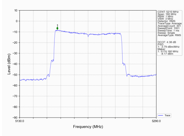
802.11ax(HEW80)_MCH_5210MHz_SU_/_Ant2_NTNV
