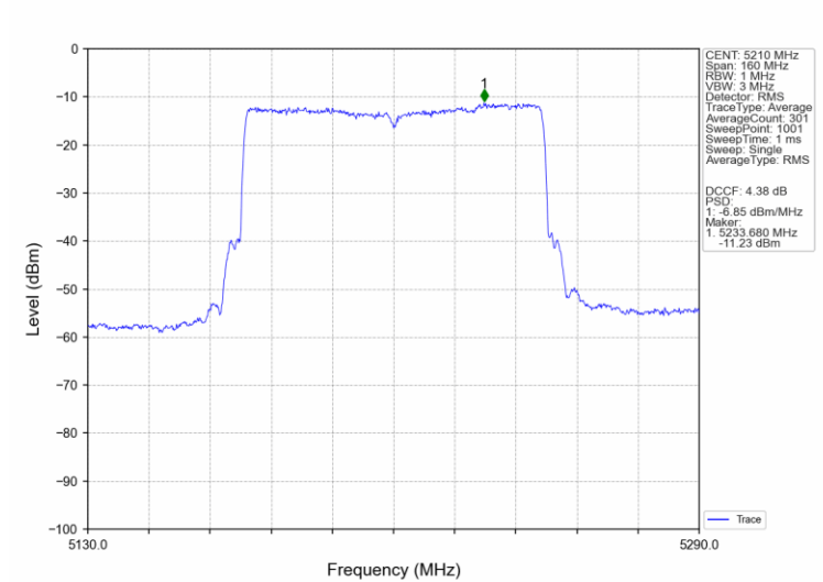
802.11ax(HEW80)_MCH_5210MHz_SU_/_Ant2_NTNV
