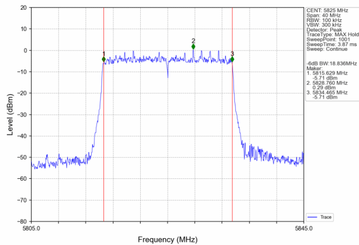
802.11ax(HEW20)_HCH_5825MHz_SU_/_Ant1_NTNV
