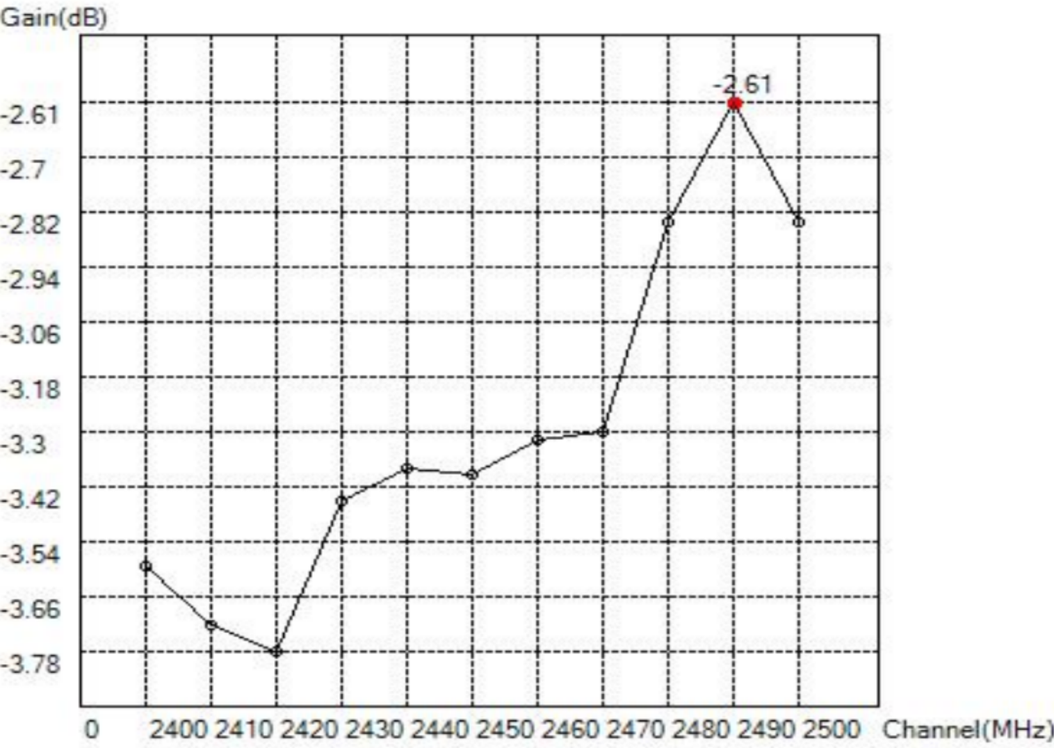
Gain-Plane
