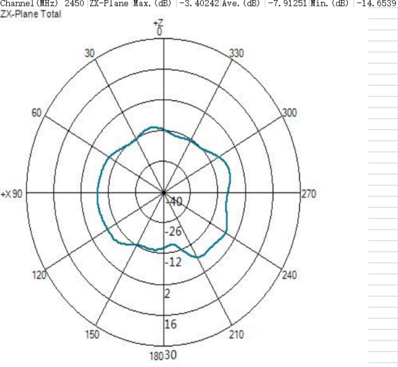
Gain-Plane
