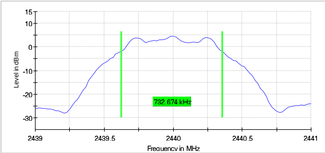
6 dB Bandwidth
