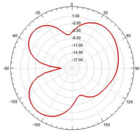
Radiation Pattern 2
