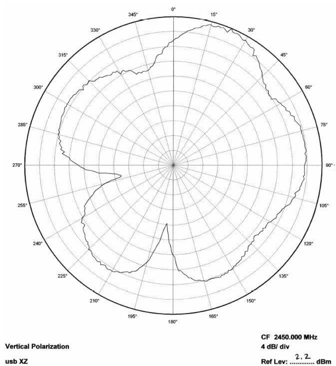
Figure 6: shows the XZ plane vertical polarization.
