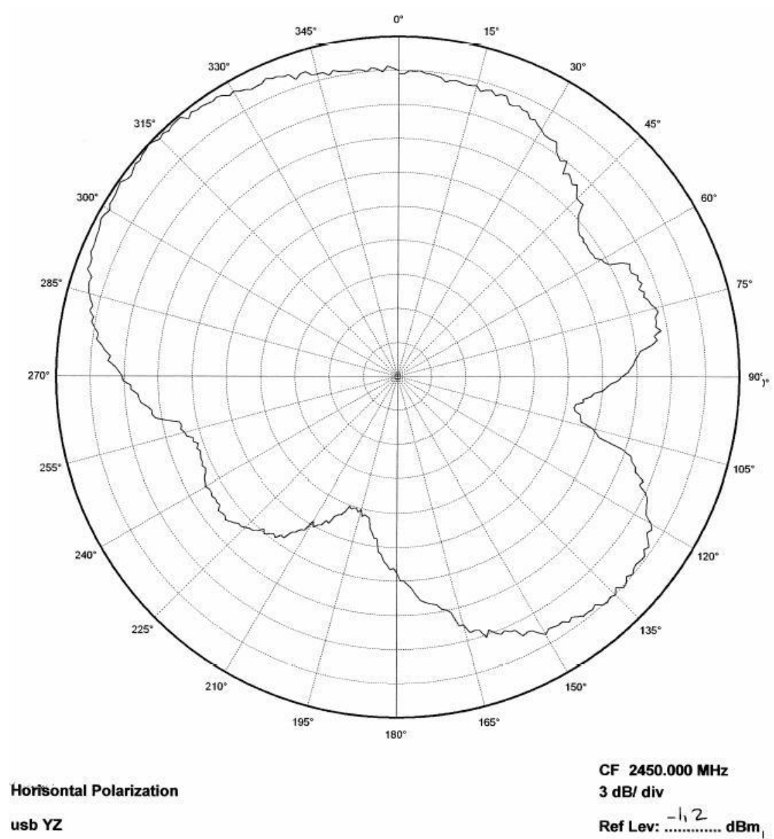
Figure 9: shows the YZ plane horizontal polarization.
