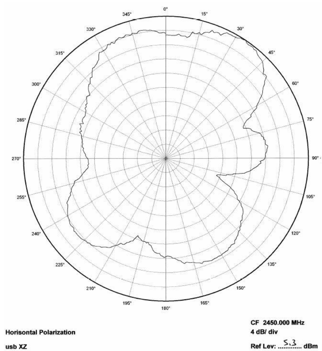
Figure 7: shows the XZ plane horizontal polarization.
