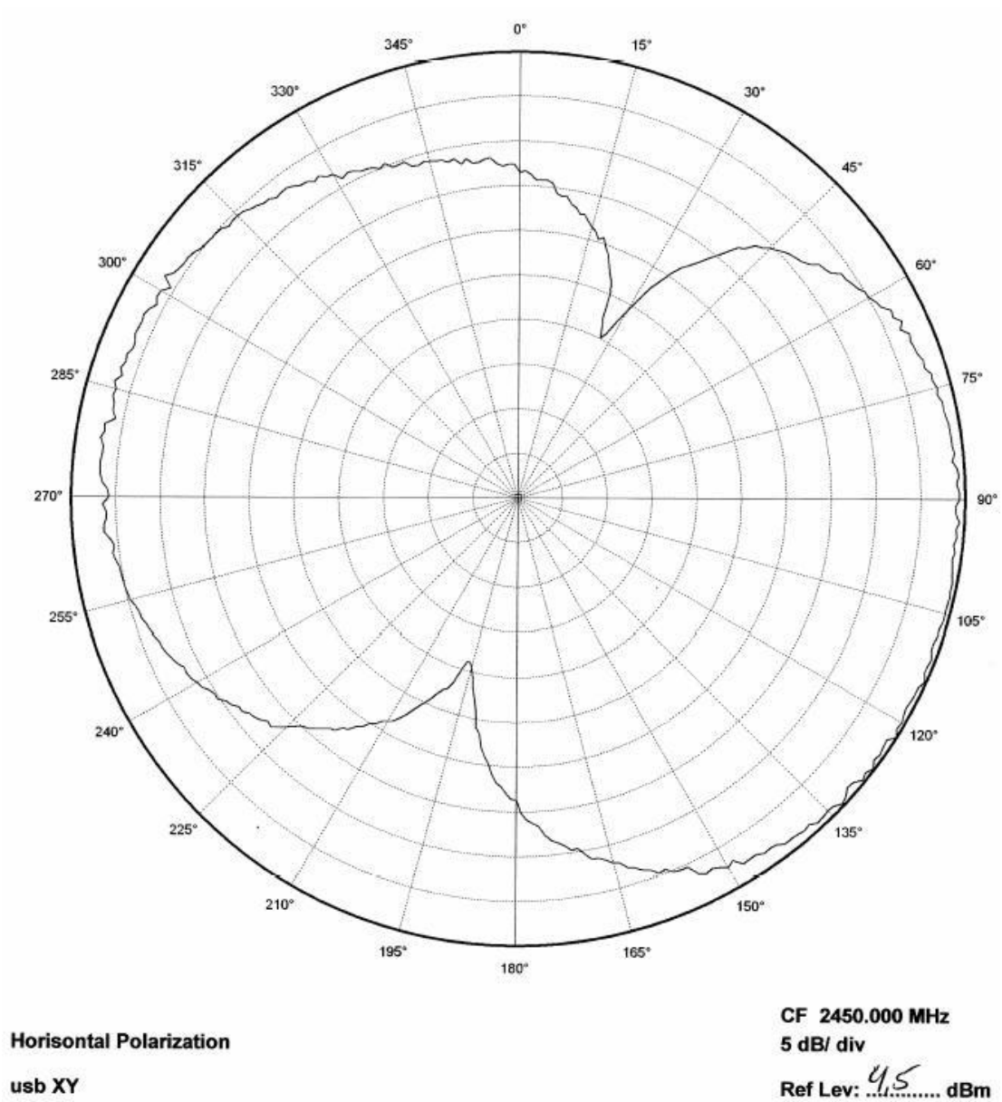
Figure 5: shows the XY plane horizontal polarization.
