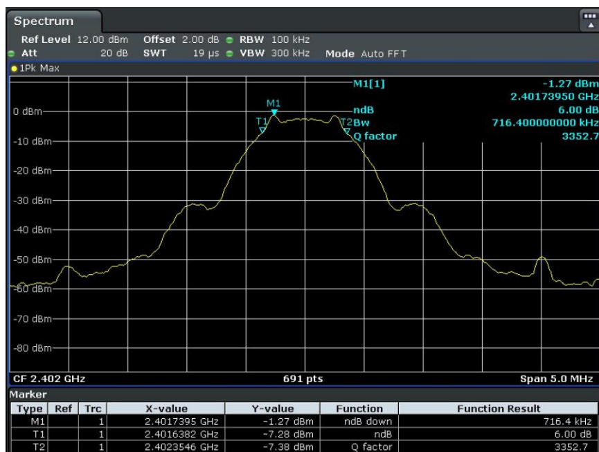
Figure 19. 6dB DTS Bandwidth: Low Channel, 2402 MHz, BLE 1 Mbps Plot
