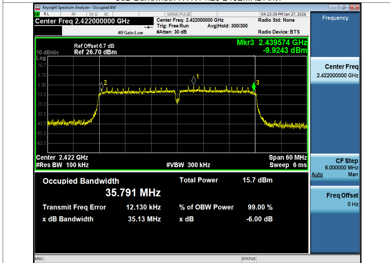
-6dB Bandwidth NVNT n40 2422MHz Ant1
