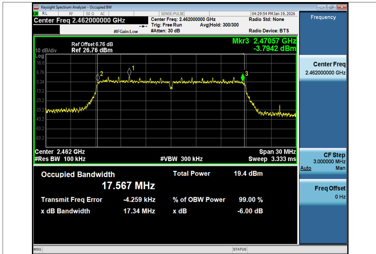
-6dB Bandwidth NVNT n20 2462MHz Ant1
