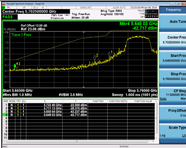
11AC20SISO-Ant1-5745-PASS
