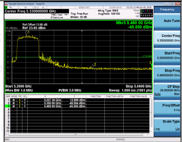
11AX40SISO-Ant1-5230-PASS
