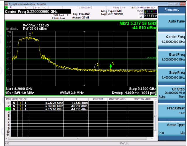
11AC40SISO-Ant1-5230-PASS
