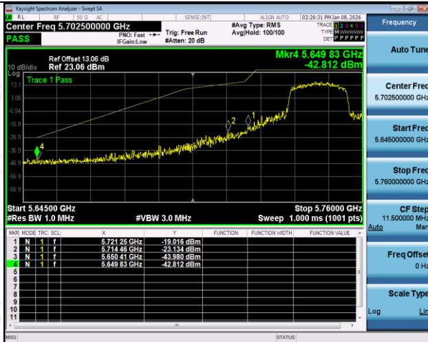
11AX20SISO-Ant1-5745-PASS
