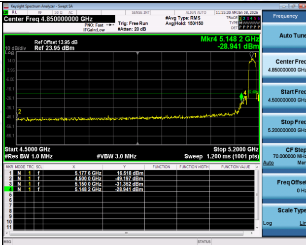
11AX20SISO-Ant1-5180-PASS
