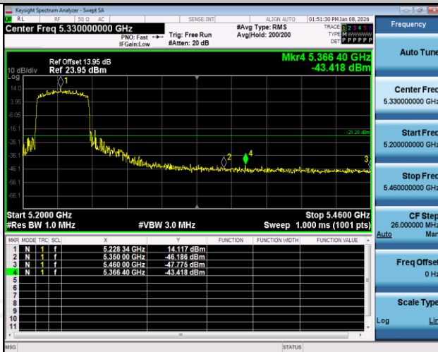
11AX40SISO-Ant1-5230-PASS
