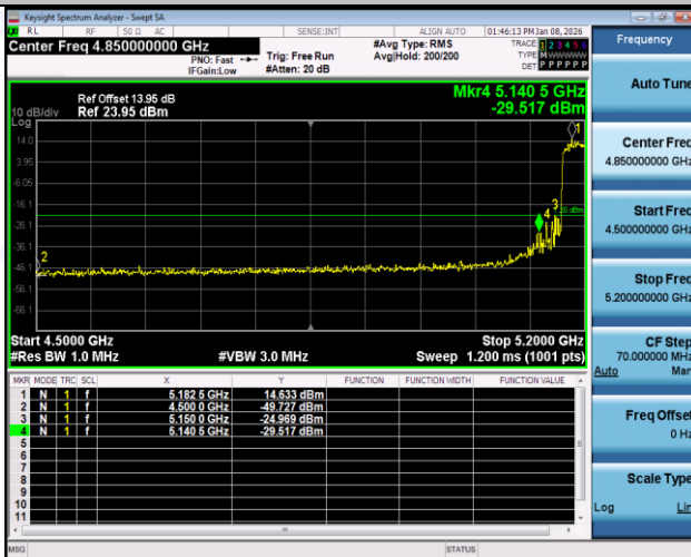
11AX40SISO-Ant1-5190-PASS
