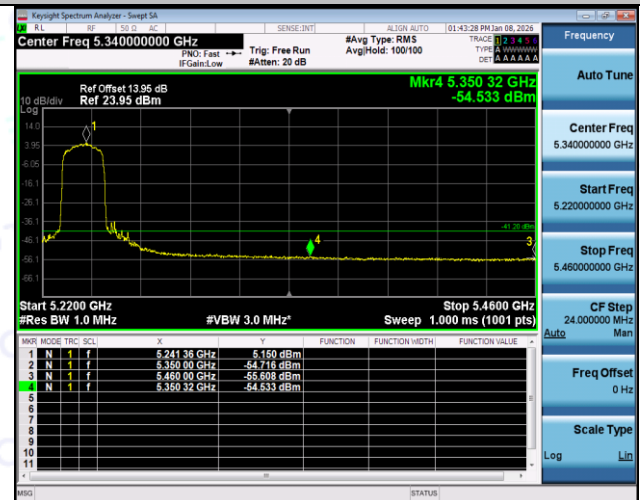
11AX20SISO-Ant1-5240-PASS
