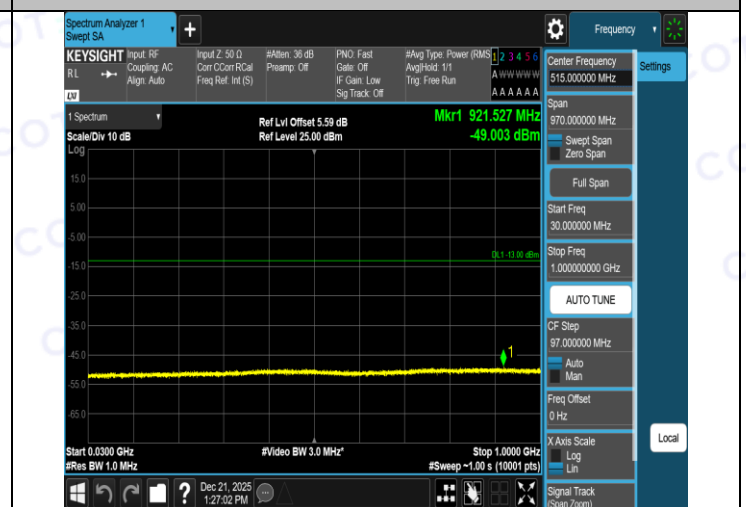
Band2-9262-4-30~1000MHz-PASS
