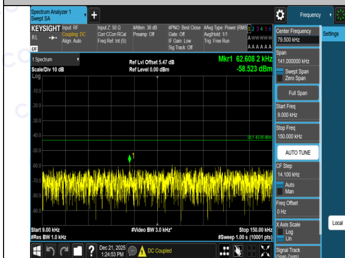
Band2-9400-3-0.009~0.15MHz-PASS
