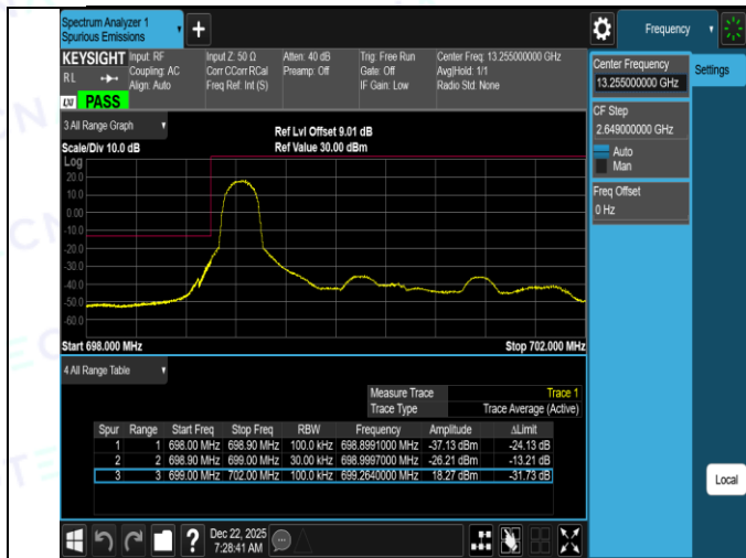
Band12-3MHz-16QAM-23025-15RB#0-PASS
