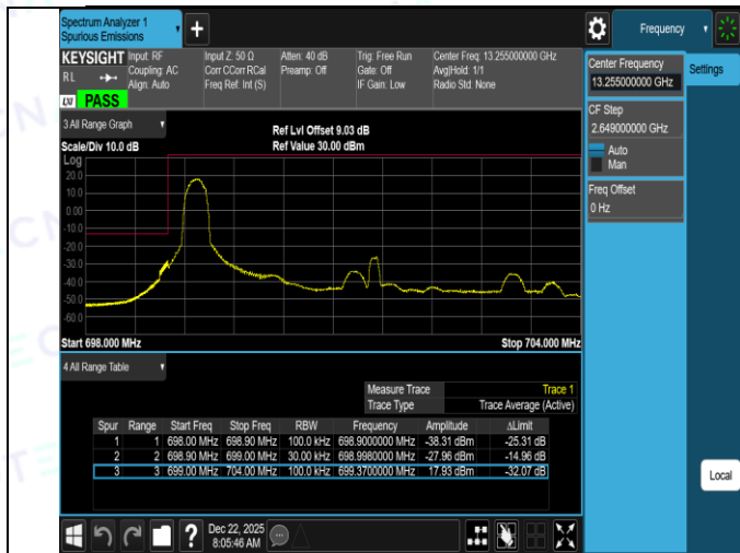
Band12-5MHz-16QAM-23035-25RB#0-PASS
