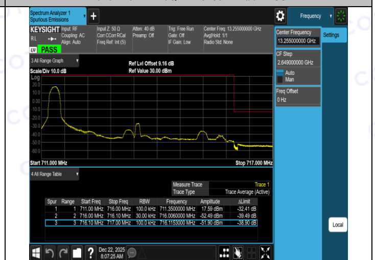
Band12-5MHz-16QAM-23155-25RB#0-PASS
