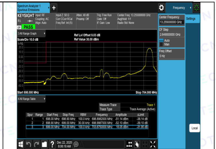
Band12-5MHz-16QAM-23155-1RB#0-PASS
