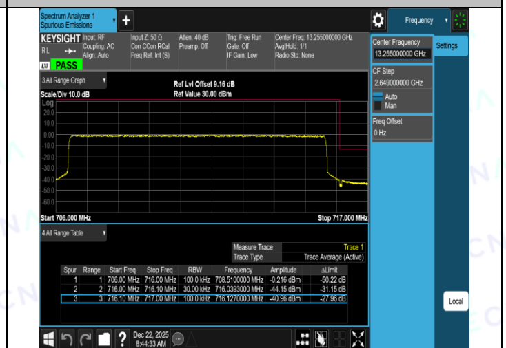
Band12-10MHz-16QAM-23060-1RB#49-PASS
