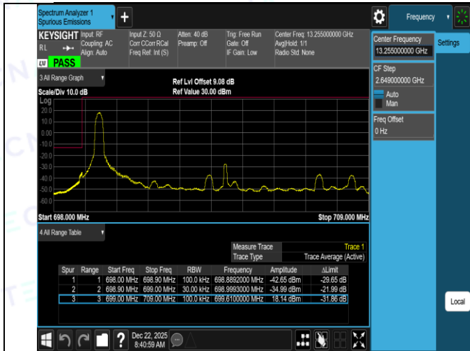
Band12-10MHz-16QAM-23060-50RB#0-PASS
