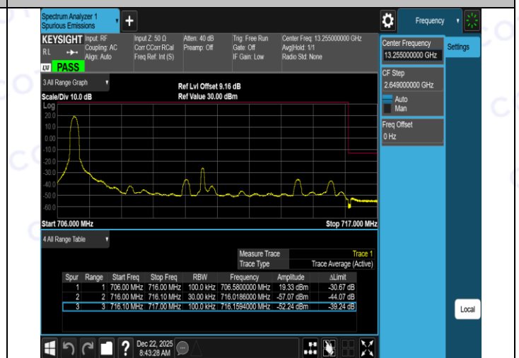
Band12-10MHz-QPSK-23130-50RB#0-PASS
