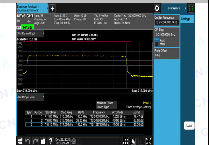
Band12-10MHz-QPSK-23060-1RB#49-PASS
