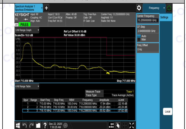
Band12-3MHz-16QAM-23165-15RB#0-PASS
