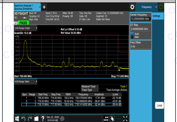
Band12-10MHz-16QAM-23130-50RB#0-PASS
