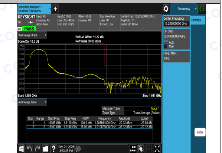
Band2-1.4MHz-16QAM-19193-6RB#0-PASS
