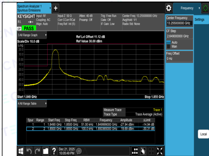
Band2-5MHz-16QAM-18625-25RB#0-PASS
