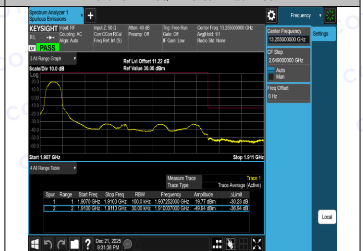
Band2-3MHz-16QAM-19185-15RB#0-PASS
