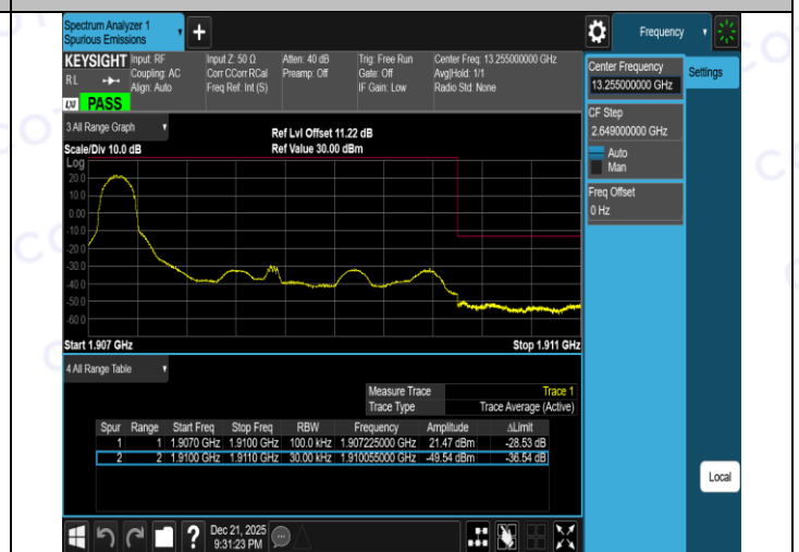
Band2-3MHz-QPSK-19185-15RB#0-PASS
