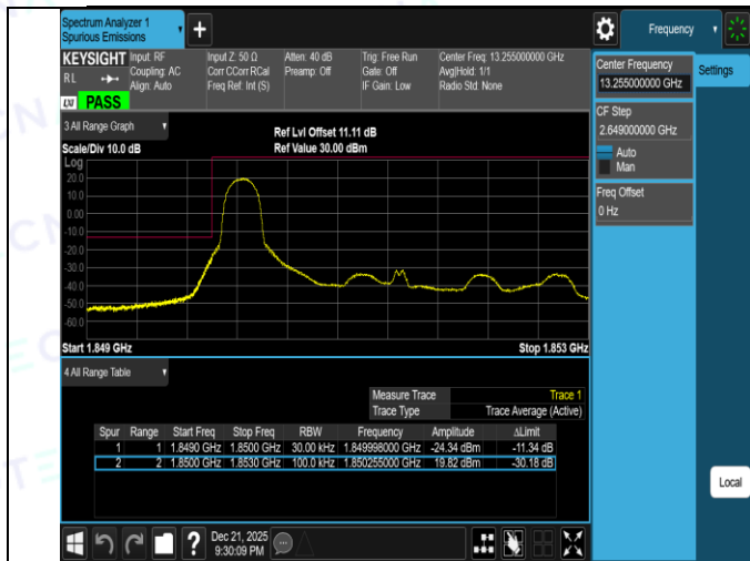
Band2-3MHz-16QAM-18615-15RB#0-PASS
