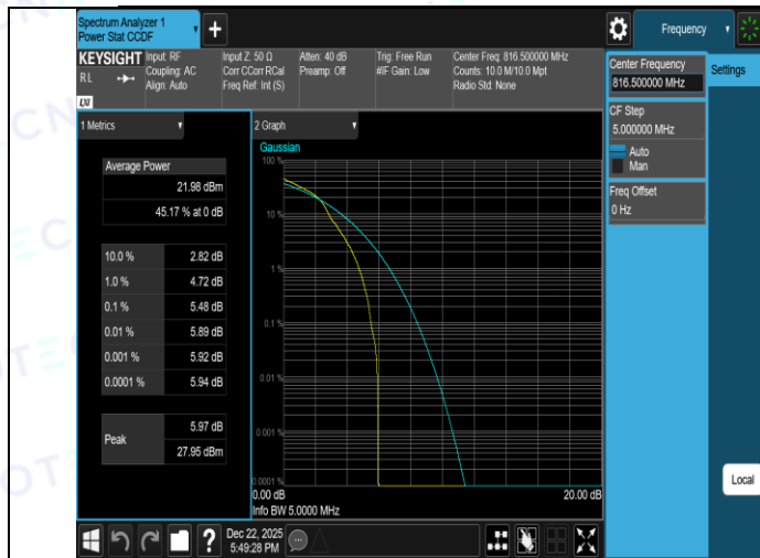
Band26(814-824)-5MHz-16QAM-26740-1RB#0-PASS
