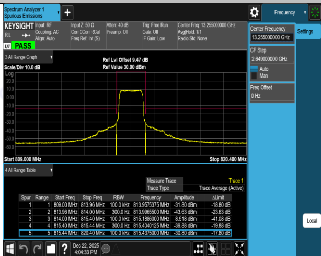
Band26(814-824)-1.4MHz-QPSK-26783-1RB#5-PASS
