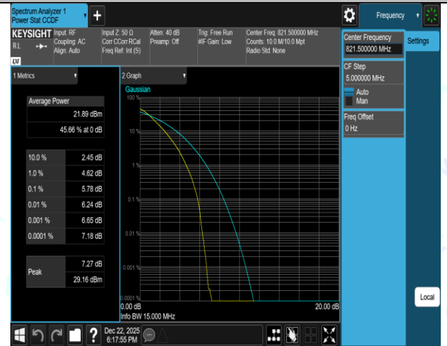
Band26(814-824)-15MHz-16QAM-26765-75RB#0-PASS
