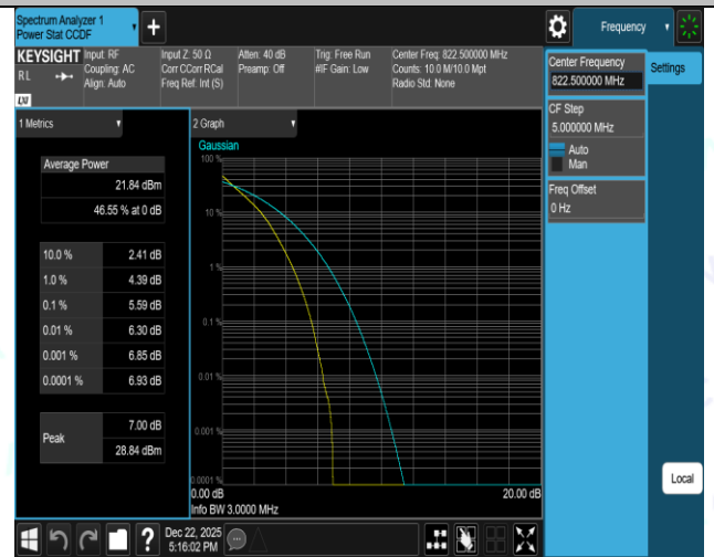
Band26(814-824)-3MHz-16QAM-26705-15RB#0-PASS
