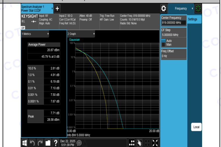
Band26(814-824)-5MHz-16QAM-26765-25RB#0-PASS
