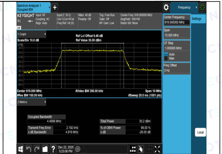
Band26(814-824)-5MHz-16QAM-26715-25RB#0-PASS
