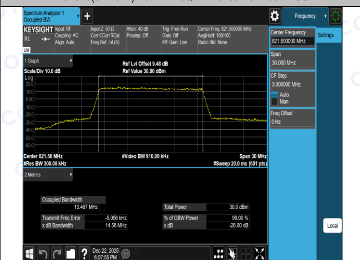
Band26(814-824)-15MHz-16QAM-26765-75RB#0-PASS
