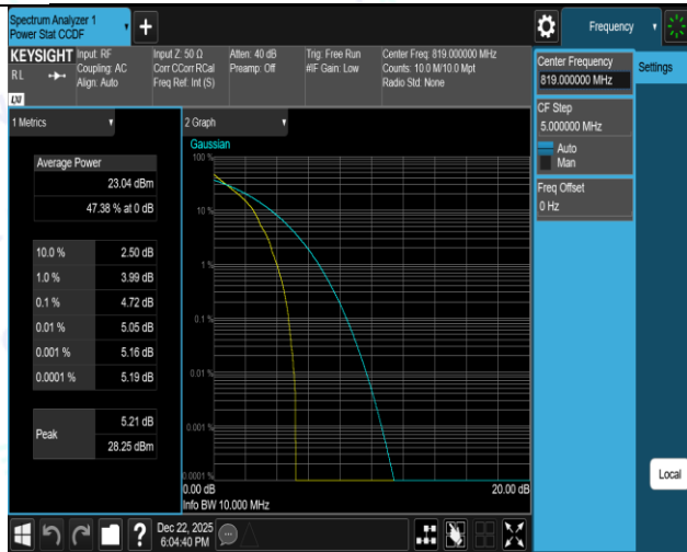
Band26(814-824)-10MHz-16QAM-26740-1RB#0-PASS
