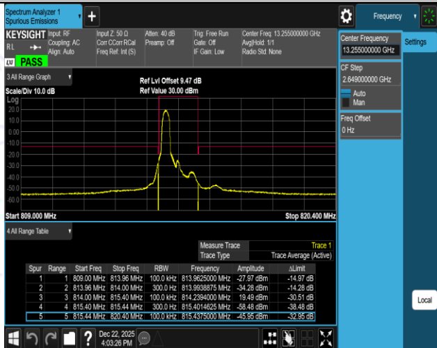
Band26(814-824)-1.4MHz-QPSK-26697-6RB#0-PASS
