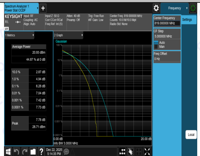
Band26(814-824)-3MHz-16QAM-26775-15RB#0-PASS
