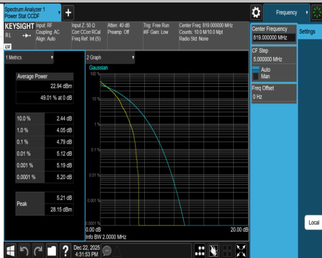
Band26(814-824)-1.4MHz-QPSK-26783-1RB#0-PASS
