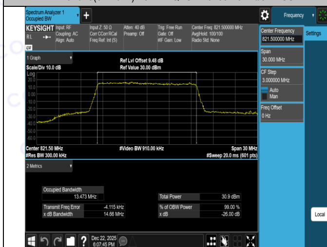
Band26(814-824)-15MHz-QPSK-26765-75RB#0-PASS
