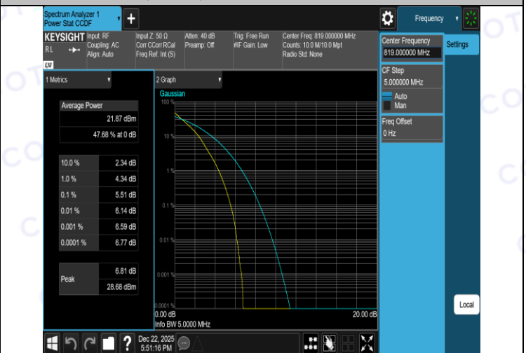
Band26(814-824)-5MHz-QPSK-26765-25RB#0-PASS
