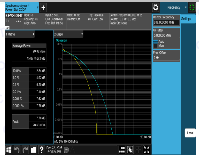
Band26(814-824)-15MHz-QPSK-26765-75RB#0-PASS
