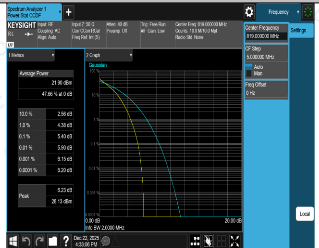
Band26(814-824)-1.4MHz-QPSK-26783-6RB#0-PASS
