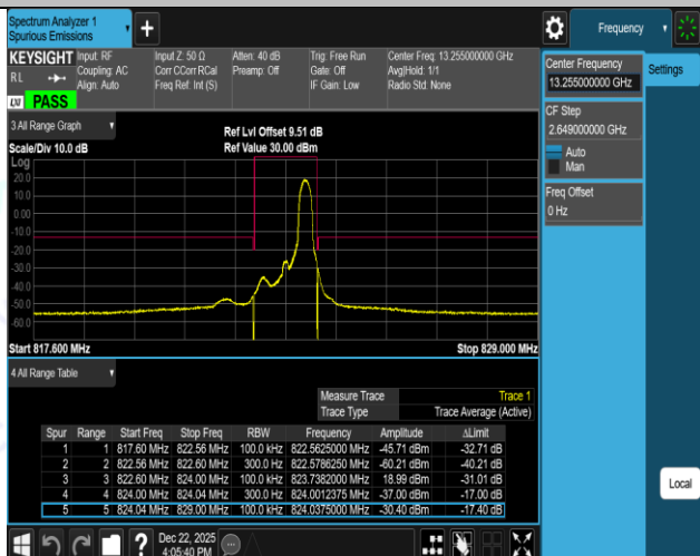
Band26(814-824)-1.4MHz-16QAM-26697-1RB#0-PASS
