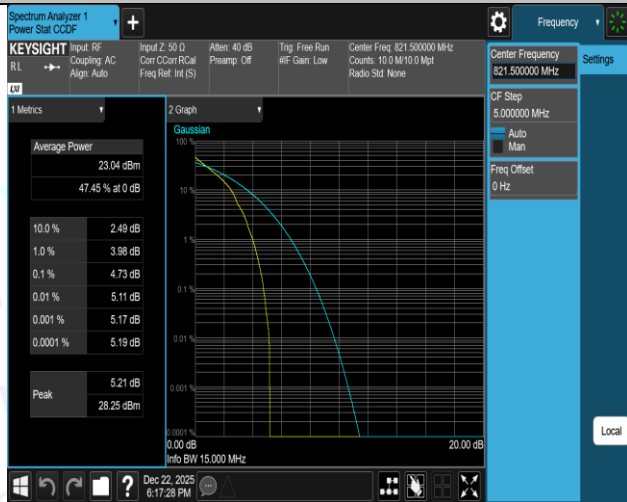
Band26(814-824)-15MHz-16QAM-26765-1RB#0-PASS
