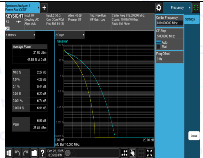
Band26(814-824)-10MHz-16QAM-26740-50RB#0-PASS
