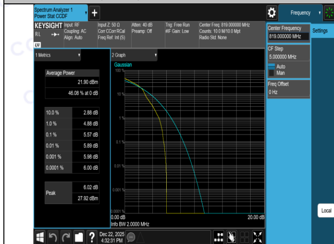
Band26(814-824)-1.4MHz-16QAM-26783-1RB#0-PASS
