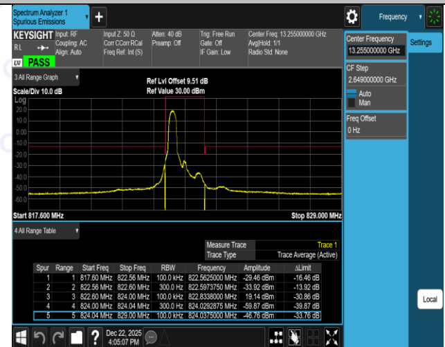
Band26(814-824)-1.4MHz-QPSK-26783-6RB#0-PASS
