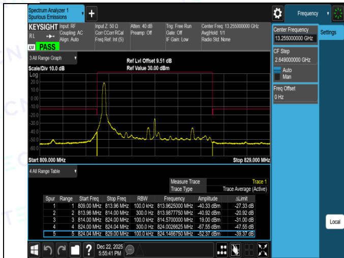
Band26(814-824)-10MHz-QPSK-26740-50RB#0-PASS
