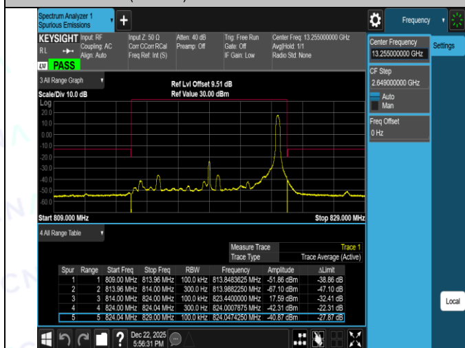
Band26(814-824)-15MHz-QPSK-26765-1RB#0-PASS
