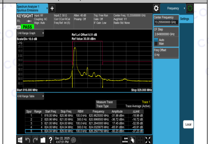
Band26(814-824)-3MHz-16QAM-26775-15RB#0-PASS
