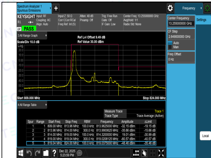
Band26(814-824)-5MHz-QPSK-26715-25RB#0-PASS
