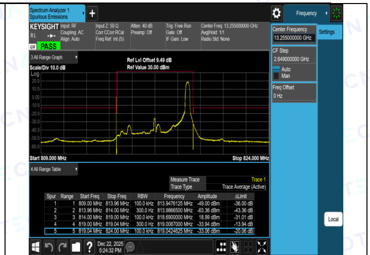
Band26(814-824)-5MHz-QPSK-26765-1RB#0-PASS
