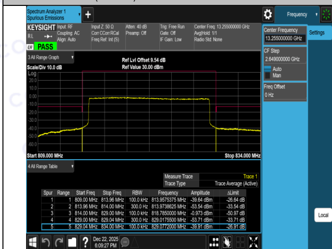
Band26(814-824)-15MHz-16QAM-26765-1RB#74-PASS
