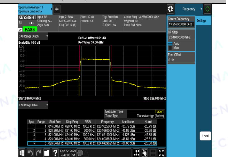
Band26(814-824)-5MHz-QPSK-26715-1RB#24-PASS
