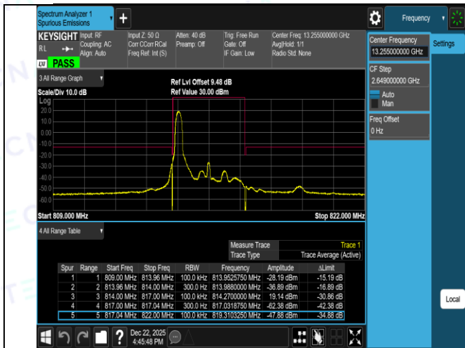
Band26(814-824)-3MHz-QPSK-26705-15RB#0-PASS
