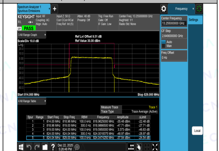
Band26(814-824)-5MHz-16QAM-26715-1RB#24-PASS
