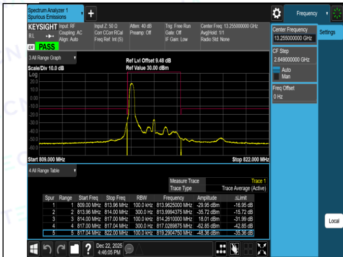
Band26(814-824)-3MHz-16QAM-26705-15RB#0-PASS
