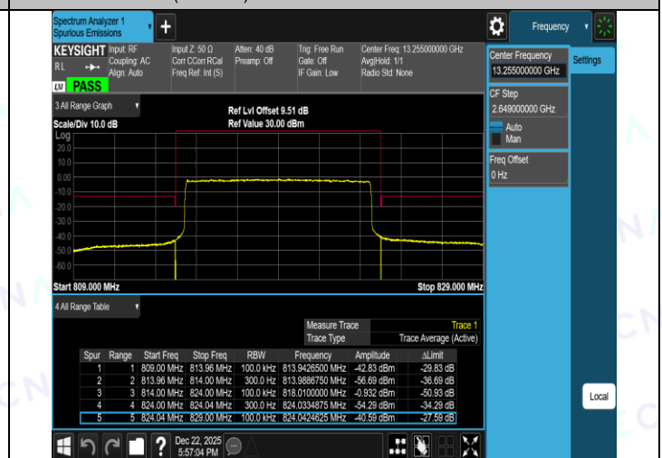
Band26(814-824)-15MHz-QPSK-26765-1RB#74-PASS
