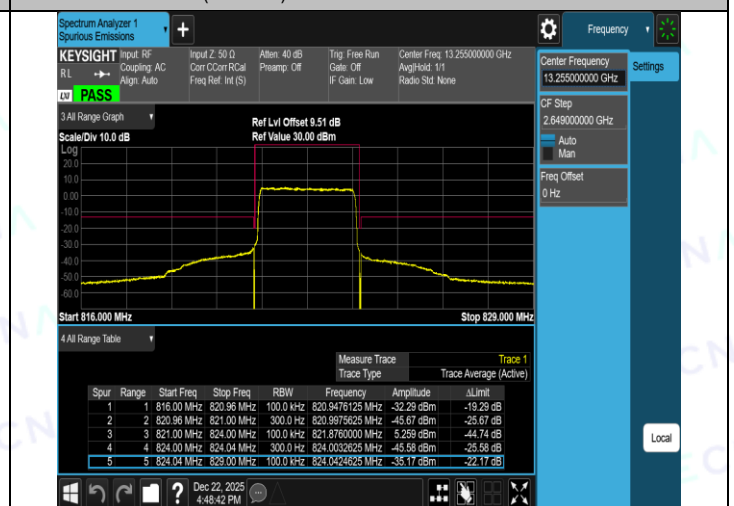
Band26(814-824)-3MHz-16QAM-26705-1RB#14-PASS
