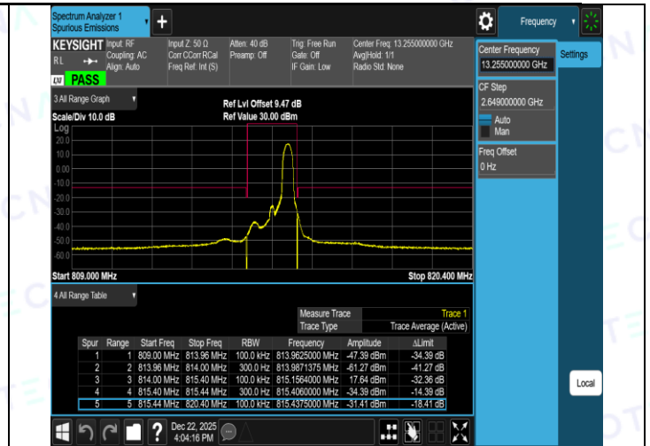
Band26(814-824)-1.4MHz-16QAM-26783-1RB#0-PASS
