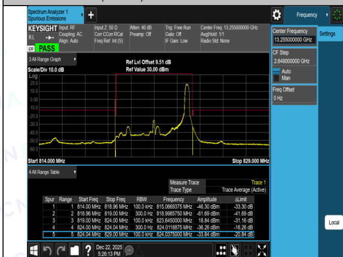
Band26(814-824)-5MHz-16QAM-26715-1RB#0-PASS
