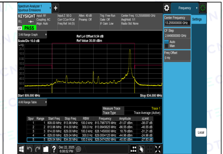
Band26(814-824)-15MHz-16QAM-26765-1RB#0-PASS
