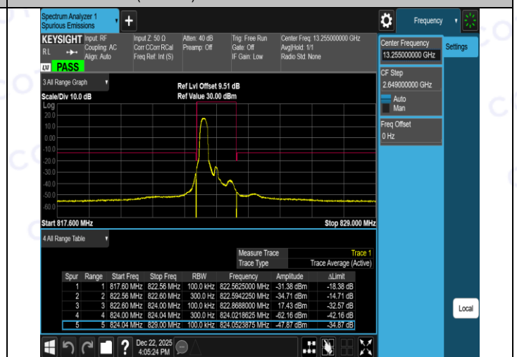
Band26(814-824)-1.4MHz-16QAM-26783-6RB#0-PASS
