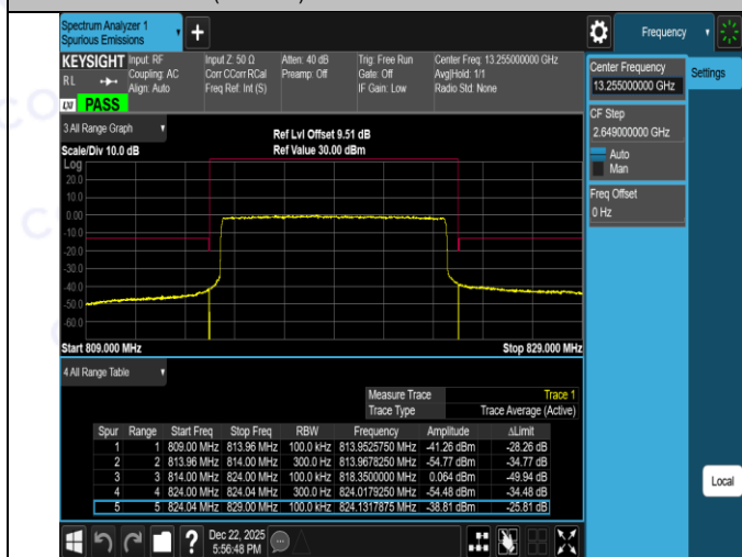
Band26(814-824)-10MHz-16QAM-26740-1RB#49-PASS
