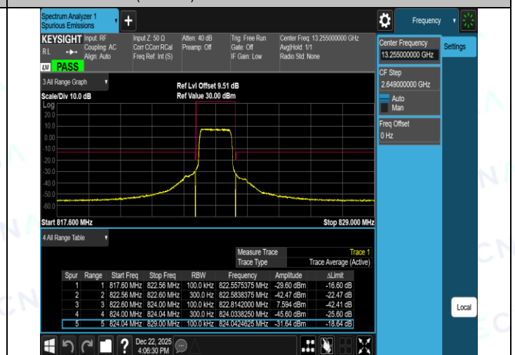
Band26(814-824)-3MHz-QPSK-26705-1RB#14-PASS
