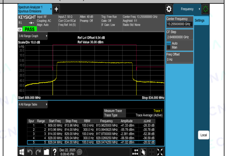
Band26(814-824)-15MHz-16QAM-26765-75RB#0-PASS
