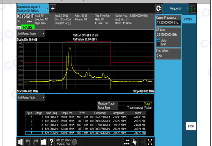
Band26(814-824)-5MHz-QPSK-26765-25RB#0-PASS
