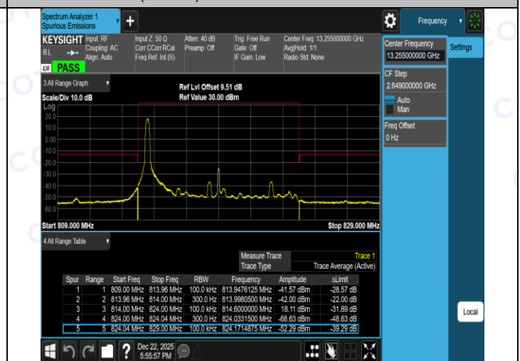
Band26(814-824)-10MHz-16QAM-26740-50RB#0-PASS
