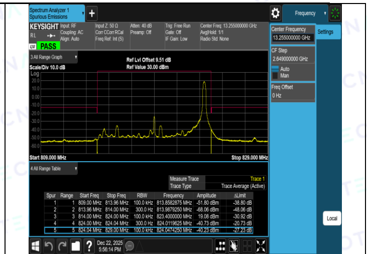
Band26(814-824)-10MHz-16QAM-26740-1RB#0-PASS
