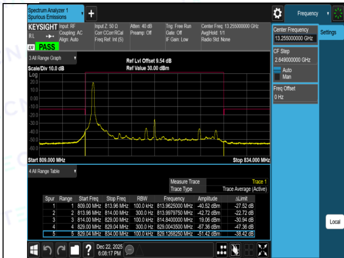
Band26(814-824)-15MHz-QPSK-26765-75RB#0-PASS
