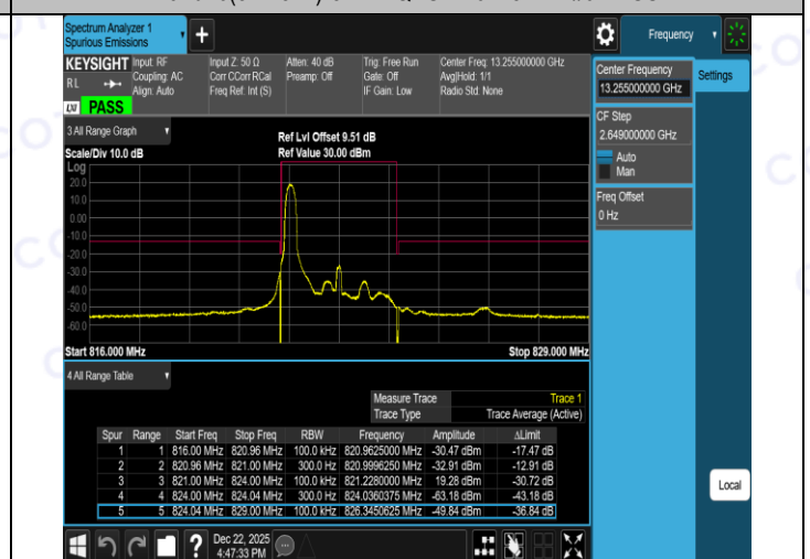
Band26(814-824)-3MHz-QPSK-26775-15RB#0-PASS
