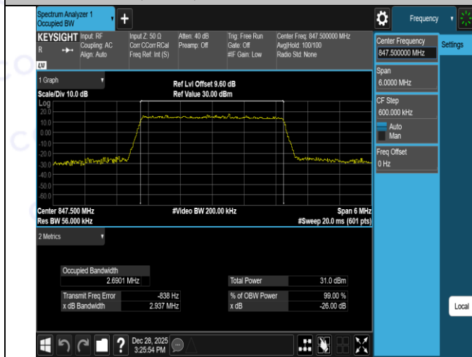
Band26(824-849)-3MHz-16QAM-26915-15RB#0-PASS
