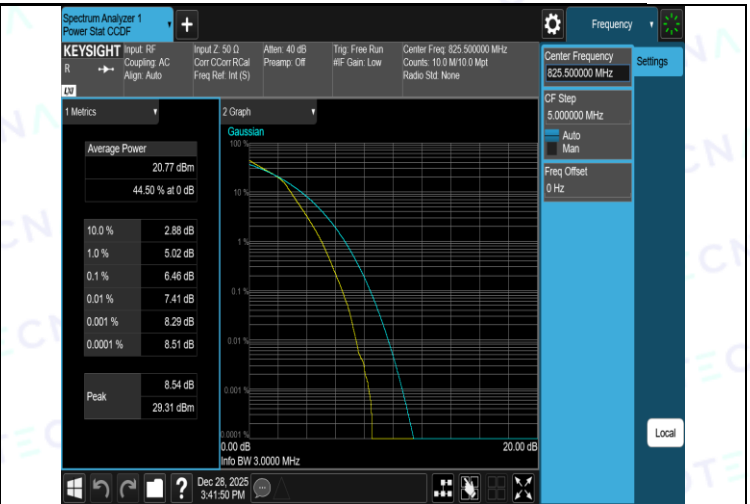
Band26(824-849)-3MHz-16QAM-26915-15RB#0-PASS
