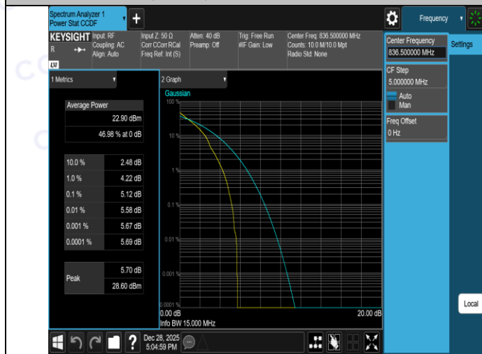
Band26(824-849)-15MHz-QPSK-26965-1RB#0-PASS
