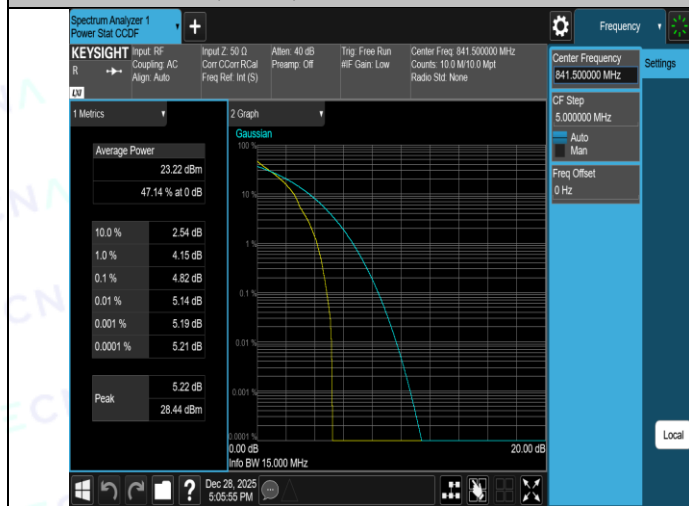
Band26(824-849)-15MHz-16QAM-26865-1RB#0-PASS
