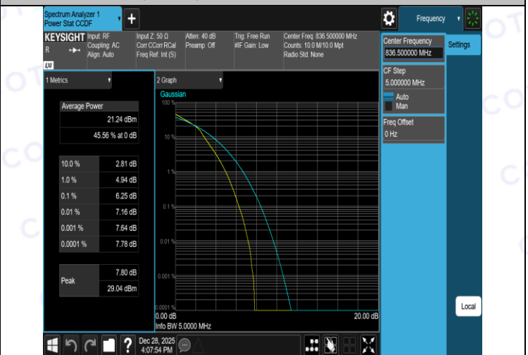
Band26(824-849)-5MHz-16QAM-27015-25RB#0-PASS
