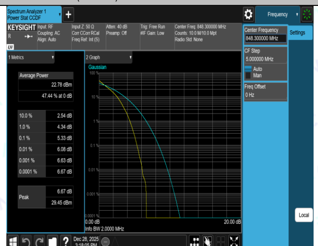
Band26(824-849)-1.4MHz-16QAM-26797-6RB#0-PASS
