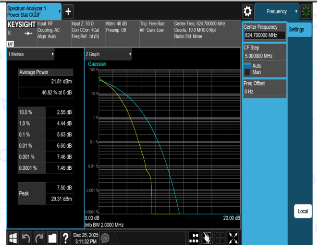
Band26(824-849)-1.4MHz-QPSK-26915-6RB#0-PASS
