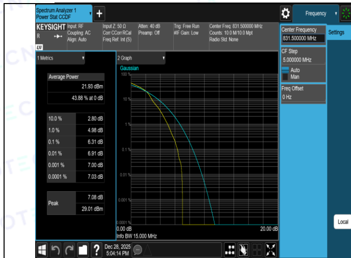
Band26(824-849)-15MHz-16QAM-26915-1RB#0-PASS
