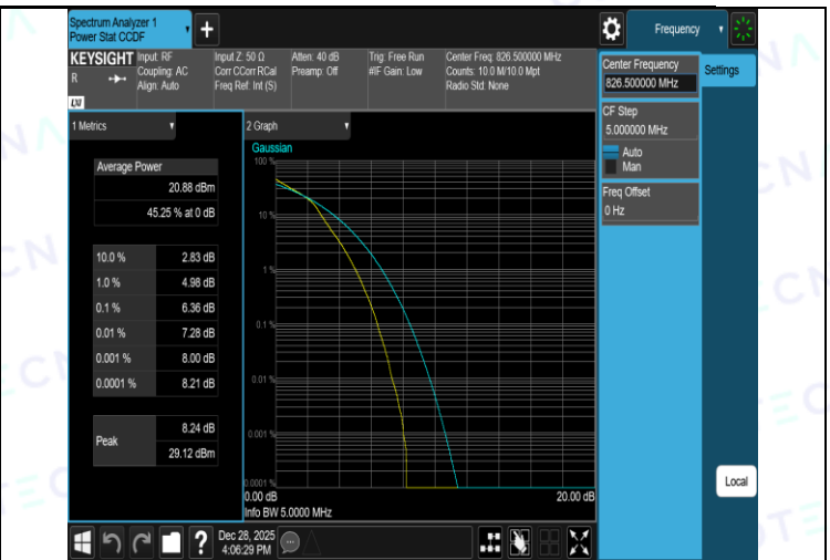
Band26(824-849)-5MHz-16QAM-26915-25RB#0-PASS
