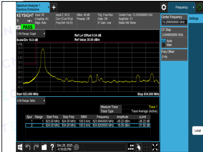
Band26(824-849)-10MHz-16QAM-26840-50RB#0-PASS
