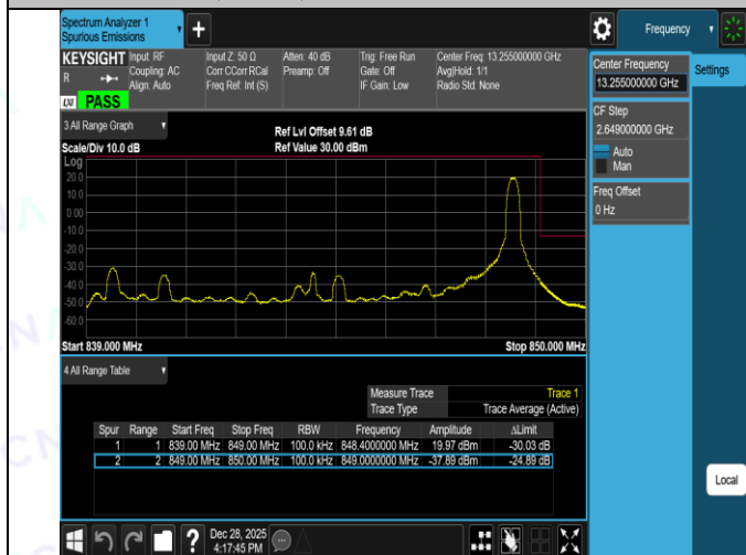
Band26(824-849)-10MHz-16QAM-26840-1RB#0-PASS
