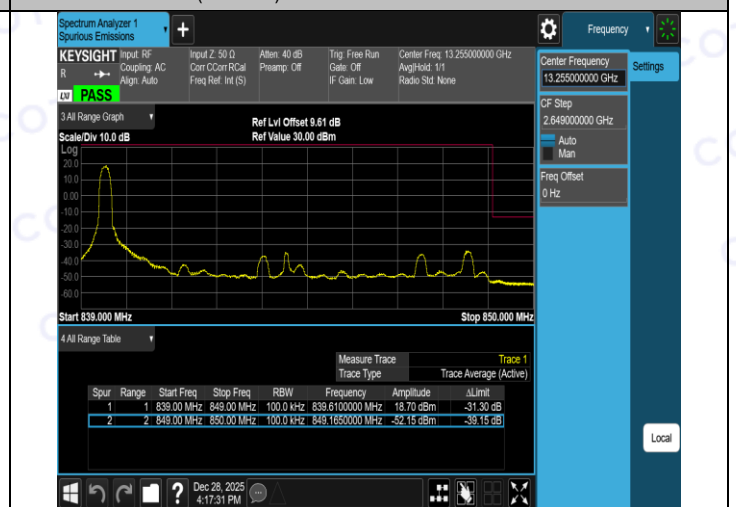
Band26(824-849)-10MHz-16QAM-26990-50RB#0-PASS
