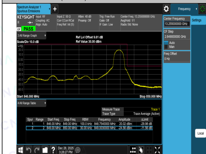
Band26(824-849)-3MHz-16QAM-26805-1RB#0-PASS
