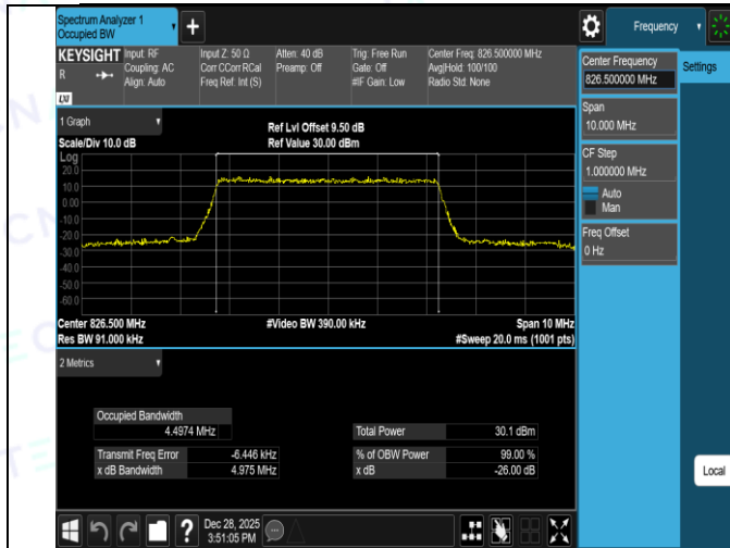
Band26(824-849)-5MHz-QPSK-27015-25RB#0-PASS
