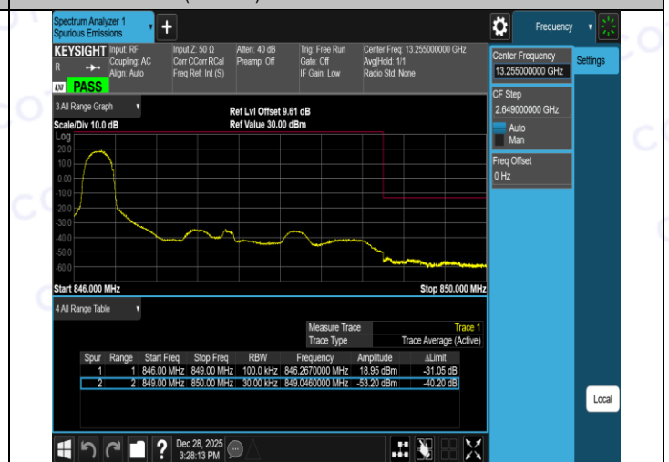
Band26(824-849)-3MHz-16QAM-27025-15RB#0-PASS
