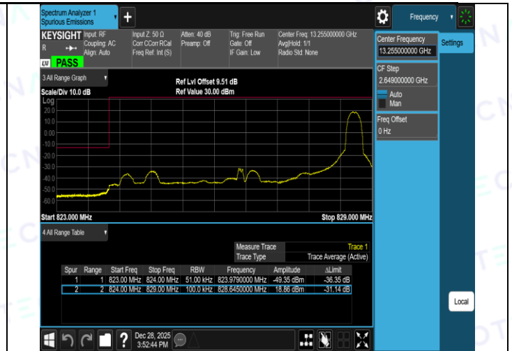
Band26(824-849)-5MHz-QPSK-27015-1RB#0-PASS
