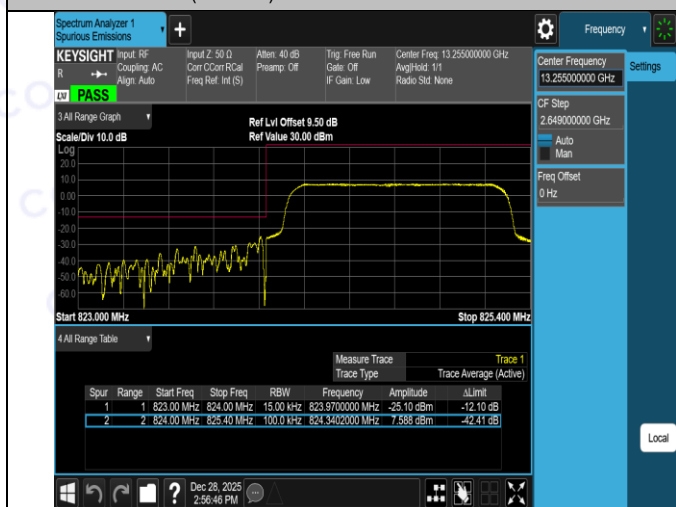
Band26(824-849)-1.4MHz-16QAM-27033-1RB#5-PASS
