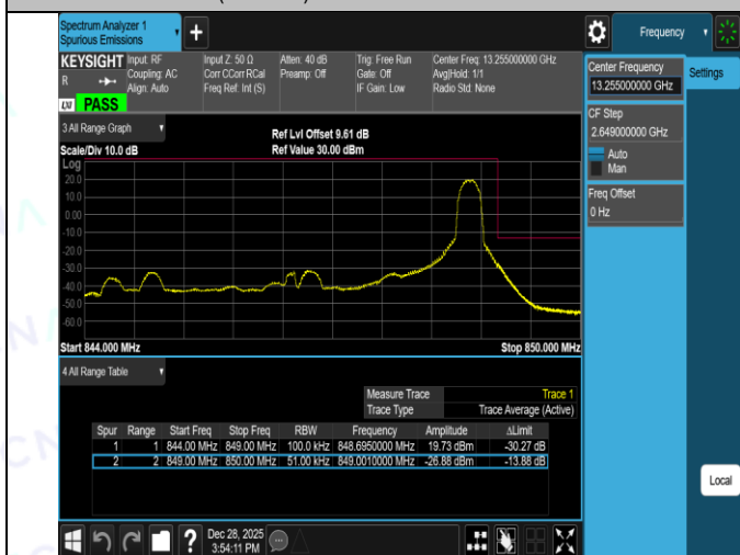
Band26(824-849)-5MHz-16QAM-26815-1RB#0-PASS
