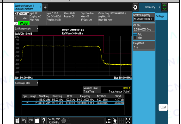
Band26(824-849)-3MHz-16QAM-26805-1RB#14-PASS
