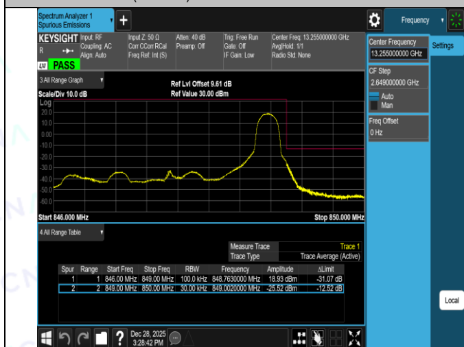
Band26(824-849)-5MHz-QPSK-26815-1RB#0-PASS
