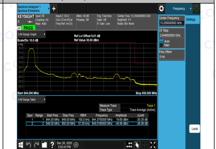
Band26(824-849)-5MHz-QPSK-27015-25RB#0-PASS
