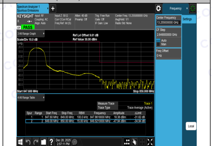
Band26(824-849)-1.4MHz-16QAM-27033-6RB#0-PASS
