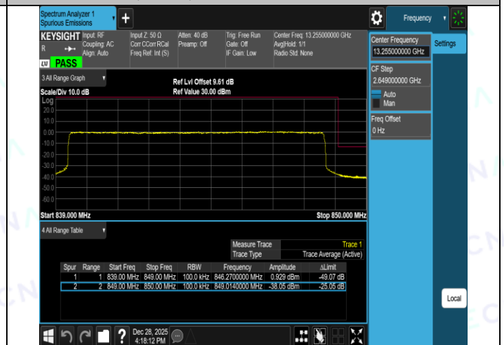
Band26(824-849)-10MHz-16QAM-26840-1RB#49-PASS
