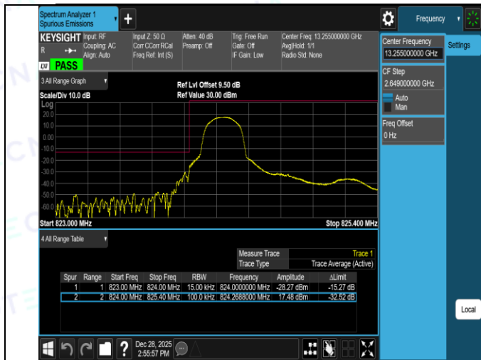
Band26(824-849)-1.4MHz-16QAM-26797-6RB#0-PASS
