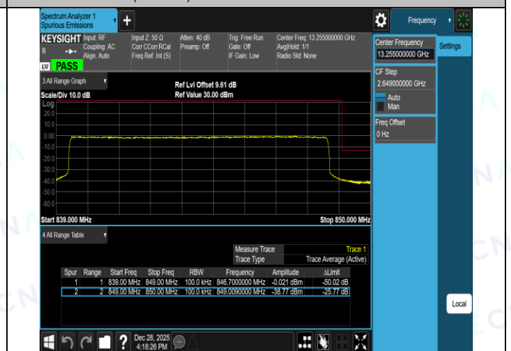
Band26(824-849)-15MHz-QPSK-26865-1RB#74-PASS
