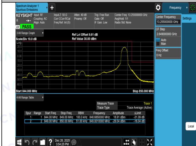
Band26(824-849)-10MHz-QPSK-26840-1RB#0-PASS
