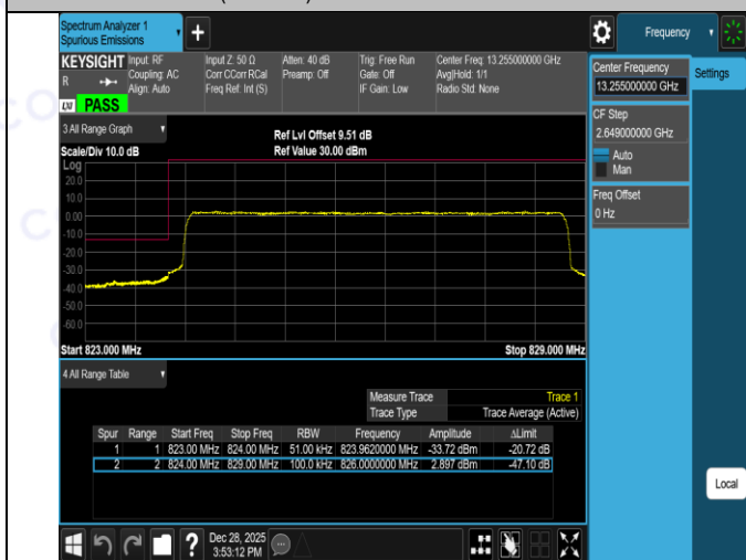
Band26(824-849)-5MHz-QPSK-27015-1RB#24-PASS
