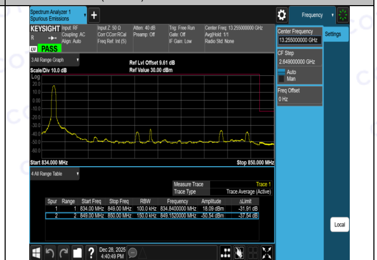
Band26(824-849)-15MHz-16QAM-26965-75RB#0-PASS
