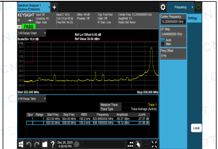
Band26(824-849)-15MHz-16QAM-26965-1RB#0-PASS
