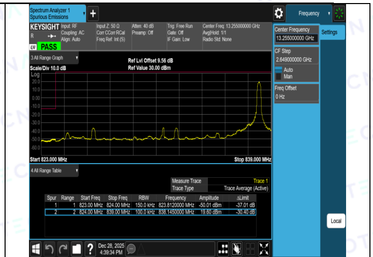
Band26(824-849)-15MHz-QPSK-26965-1RB#0-PASS
