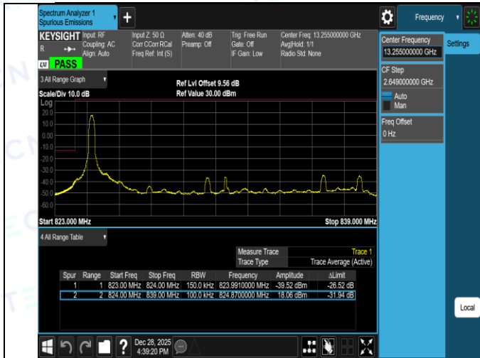
Band26(824-849)-15MHz-16QAM-26865-75RB#0-PASS
