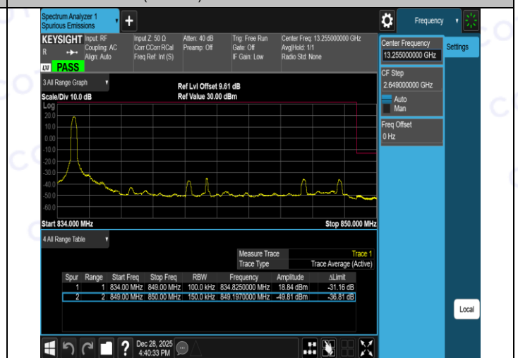
Band26(824-849)-15MHz-QPSK-26965-75RB#0-PASS
