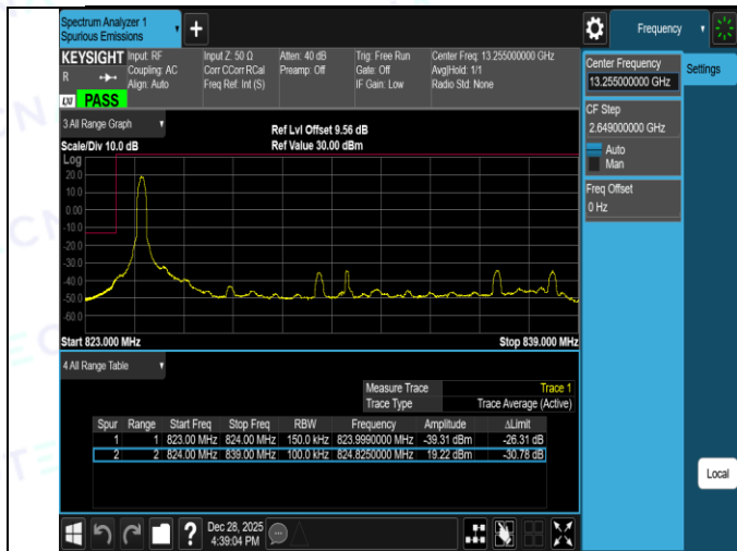
Band26(824-849)-15MHz-QPSK-26865-75RB#0-PASS
