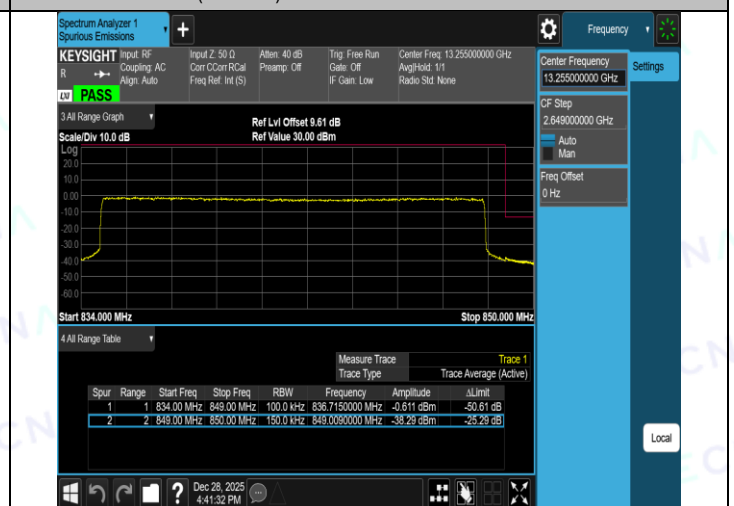
Band26(824-849)-15MHz-16QAM-26865-1RB#74-PASS
