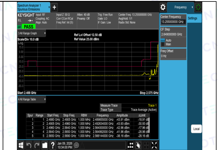
Band38-5MHz-16QAM-38225-1RB#0-PASS
