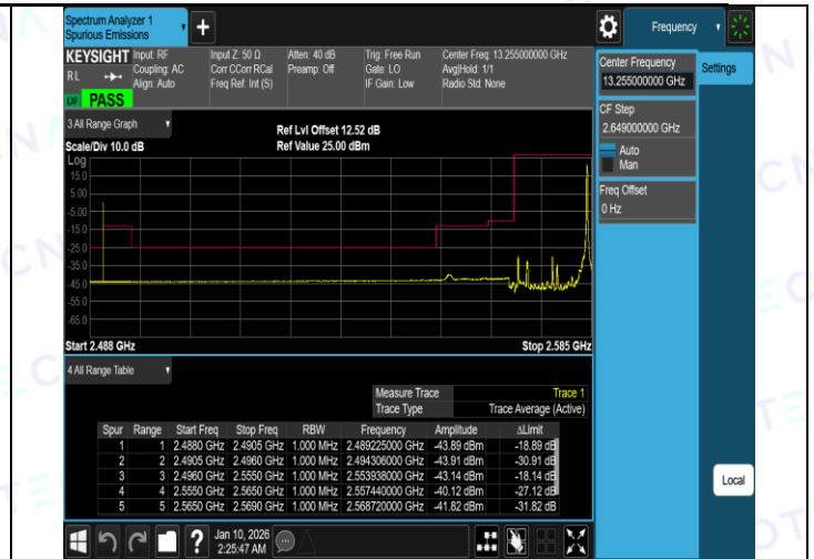
Band38-15MHz-QPSK-38175-1RB#0-PASS
