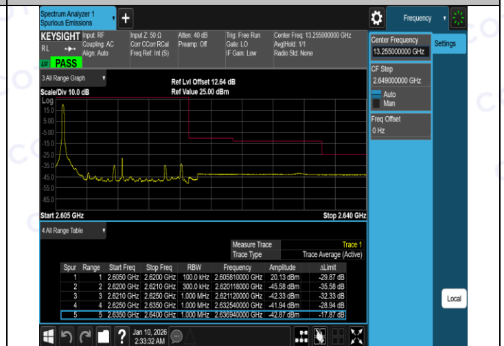
Band38-15MHz-QPSK-38175-75RB#0-PASS
