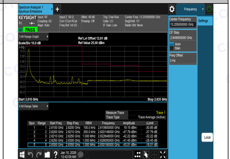
Band38-10MHz-16QAM-38200-50RB#0-PASS
