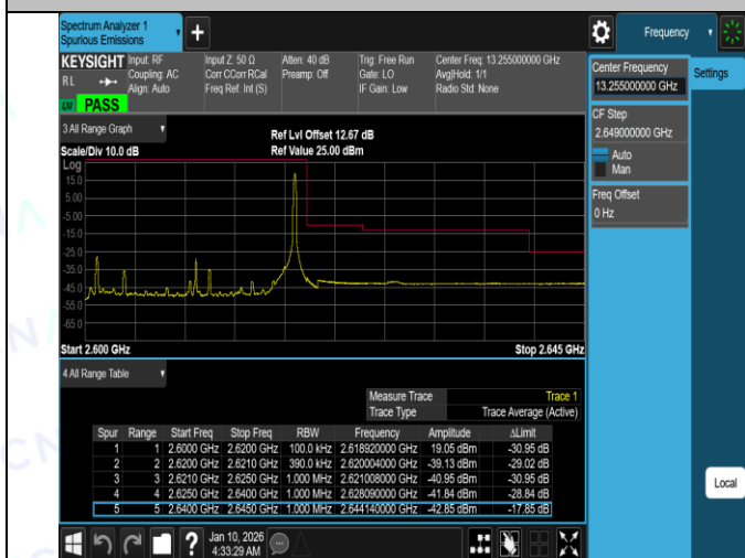
Band38-20MHz-16QAM-38150-1RB#99-PASS
