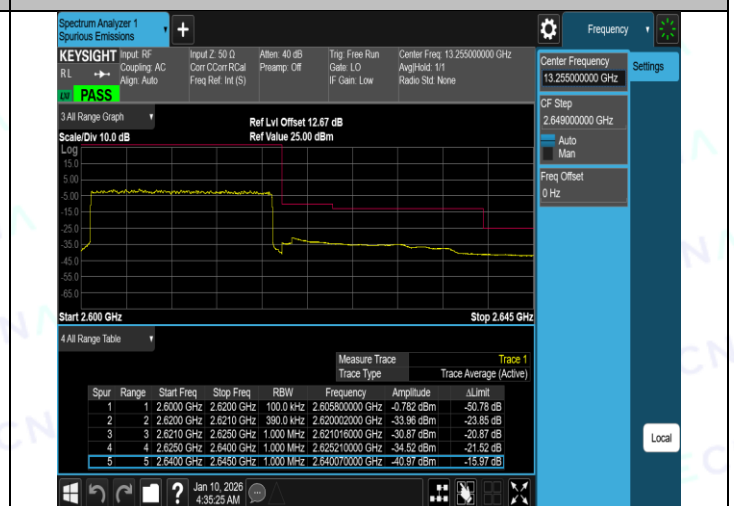
Band38-20MHz-16QAM-37850-1RB#99-PASS
