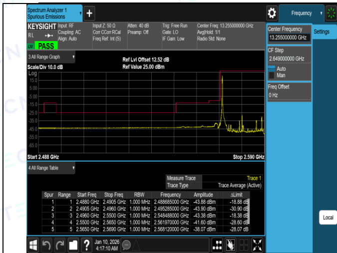
Band38-20MHz-16QAM-37850-100RB#0-PASS
