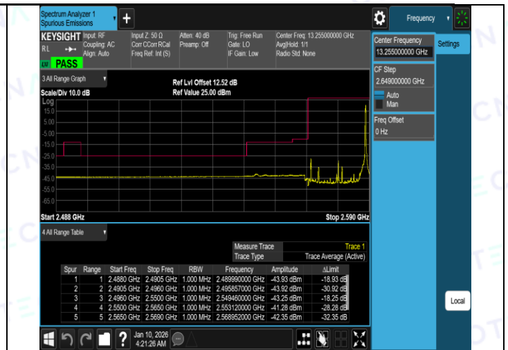
Band38-20MHz-16QAM-38150-1RB#0-PASS
