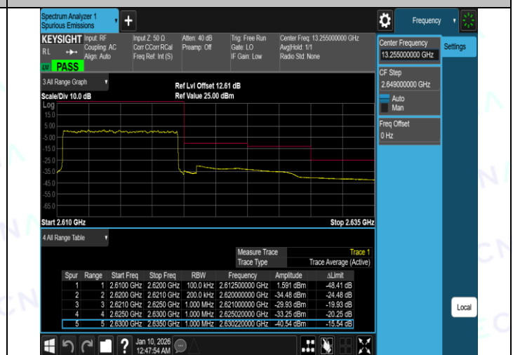
Band38-10MHz-16QAM-37800-1RB#49-PASS
