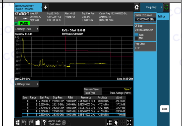
Band38-10MHz-QPSK-38200-50RB#0-PASS
