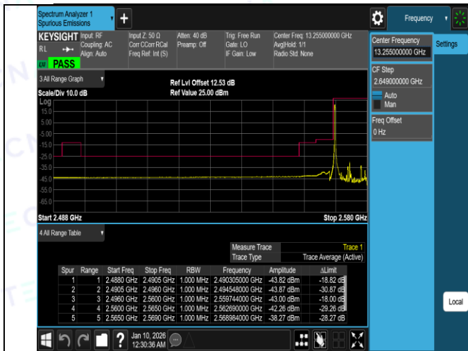
Band38-10MHz-16QAM-37800-50RB#0-PASS
