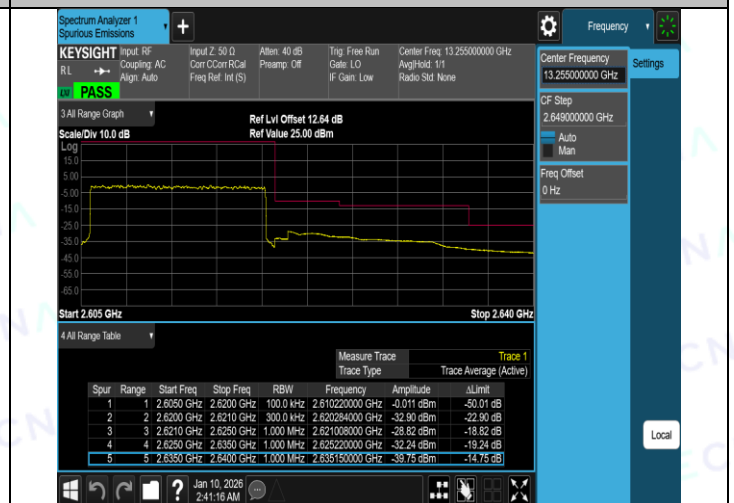
Band38-15MHz-16QAM-37825-1RB#74-PASS
