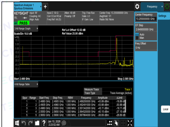
Band38-15MHz-16QAM-37825-75RB#0-PASS
