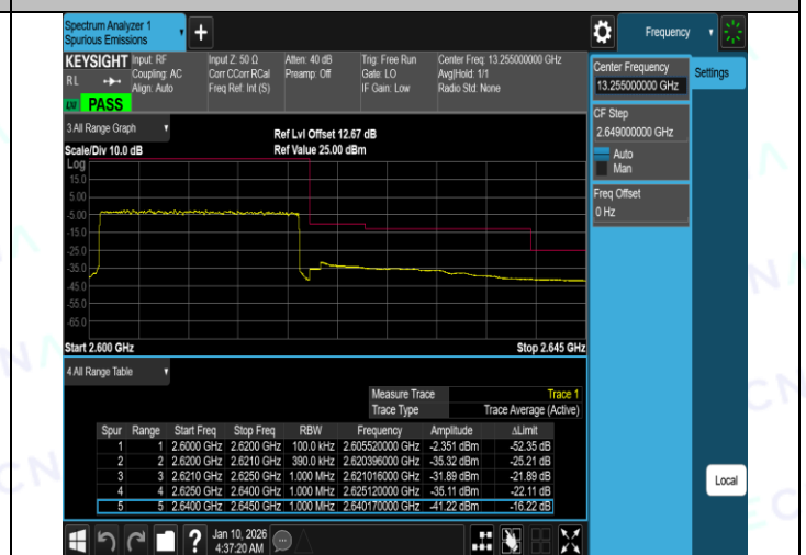
Band38-20MHz-16QAM-38150-100RB#0-PASS
