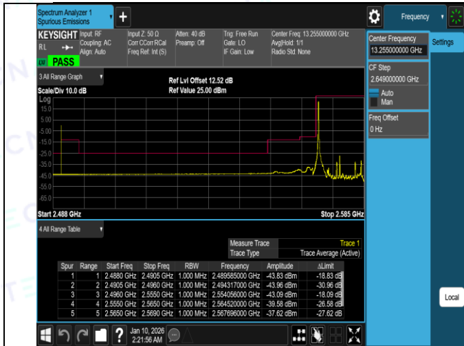
Band38-15MHz-QPSK-37825-75RB#0-PASS
