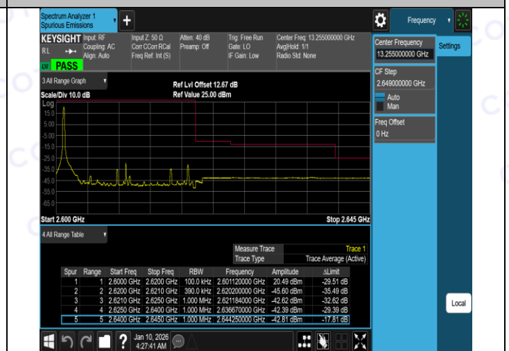
Band38-20MHz-QPSK-38150-100RB#0-PASS
