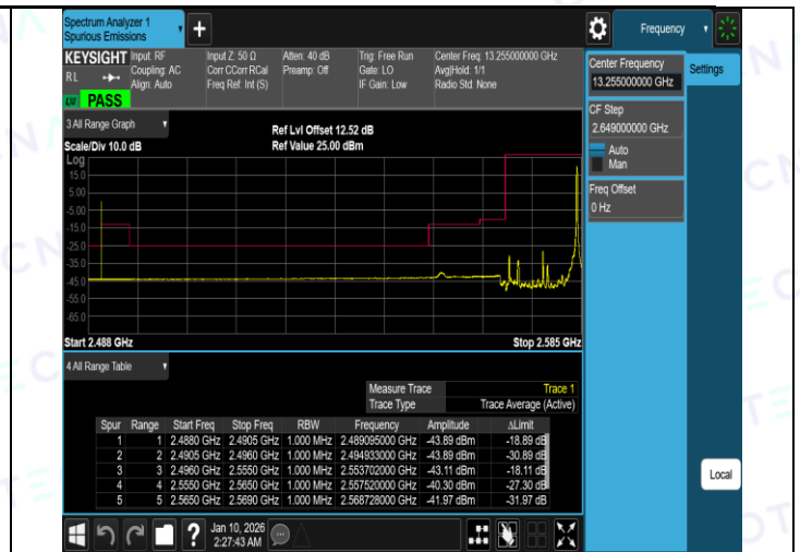
Band38-15MHz-16QAM-38175-1RB#0-PASS
