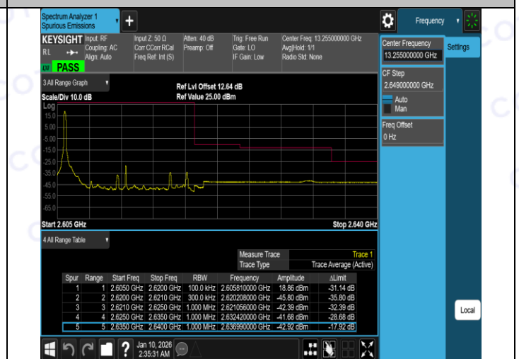
Band38-15MHz-16QAM-38175-75RB#0-PASS
