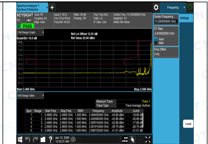
Band38-10MHz-QPSK-38200-1RB#0-PASS
