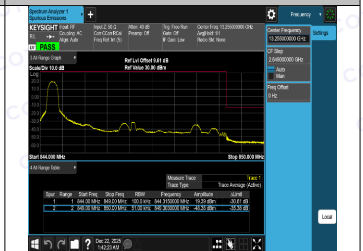
Band5-5MHz-QPSK-20625-25RB#0-PASS
