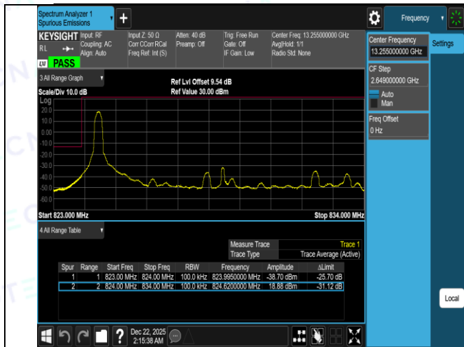
Band5-10MHz-QPSK-20450-50RB#0-PASS
