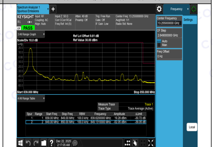
Band5-10MHz-QPSK-20600-50RB#0-PASS
